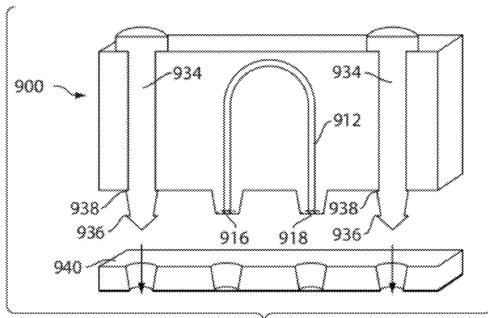
Fig. 12D
