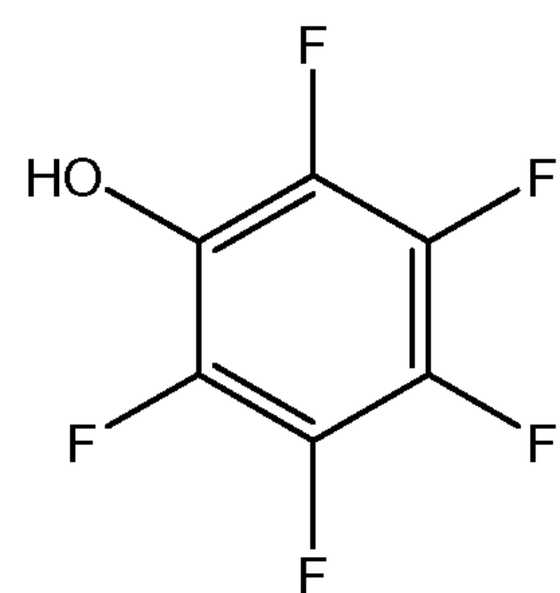
Pentafluorophenol
