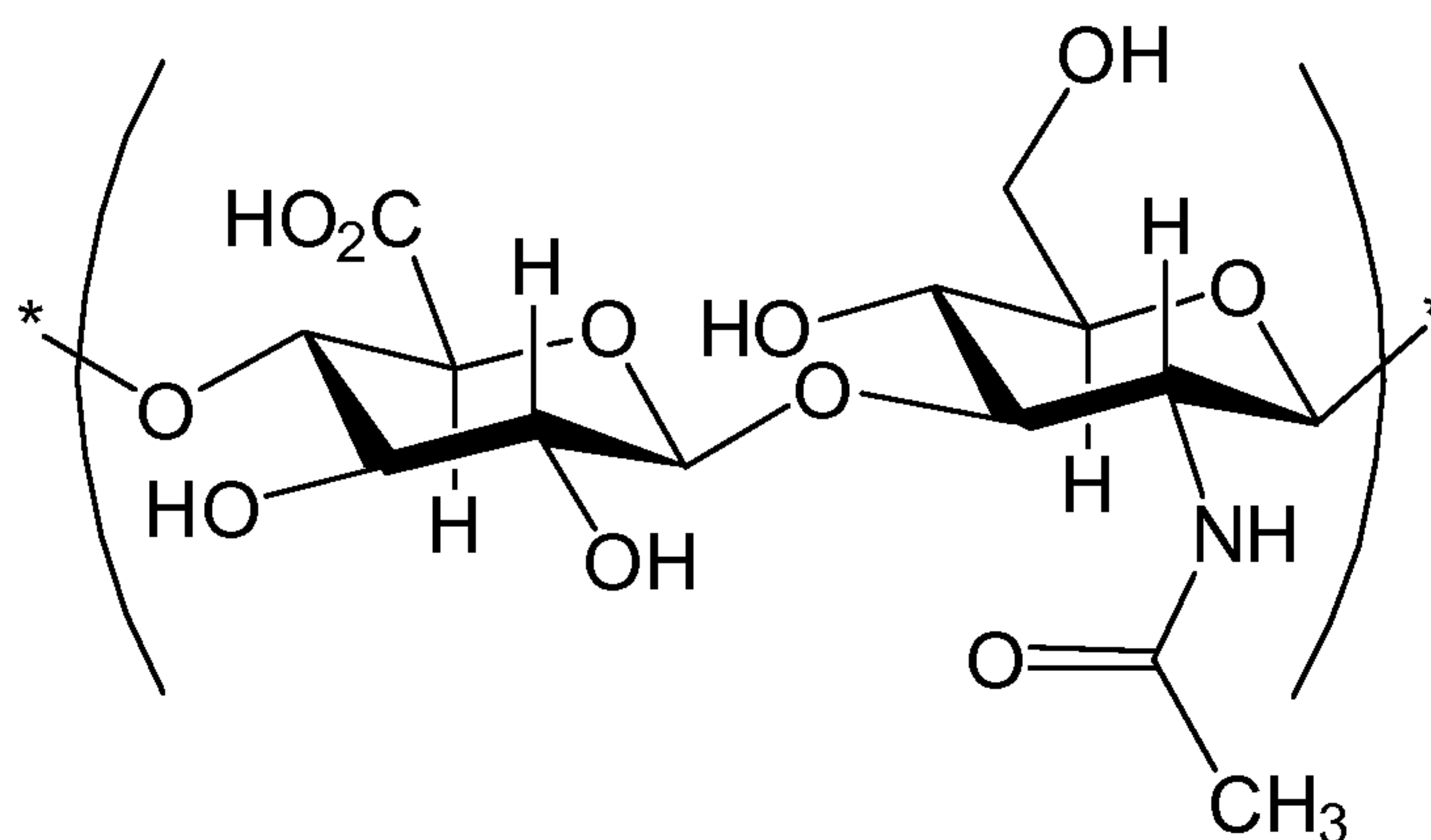
Hyaluronic acid
