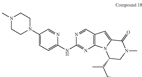
Compound 18
