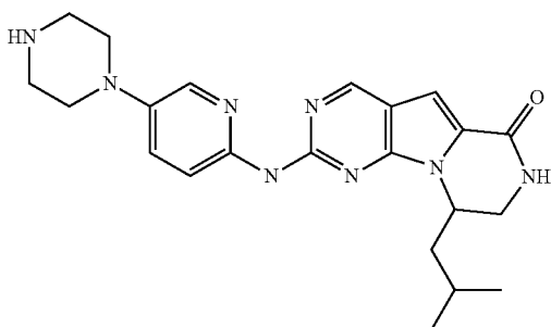
Compound 46
