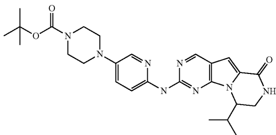
Compound 6
