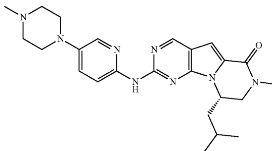
Compound 14
