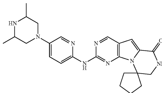
Compound 42
