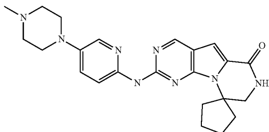
Compound 29
