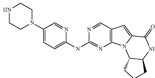
Compound 49
