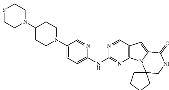
Compound 43
