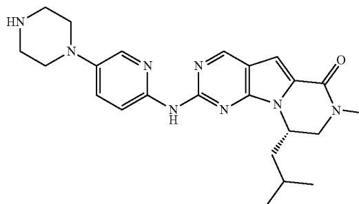
Compound 15
