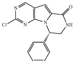
tert-butyl N-[(2S)-2-[(5-bromo-2-chloro-pyrimidin-4-yl)amino]-2-phenyl-ethyl] carbamate
