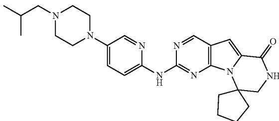
Compound 36
