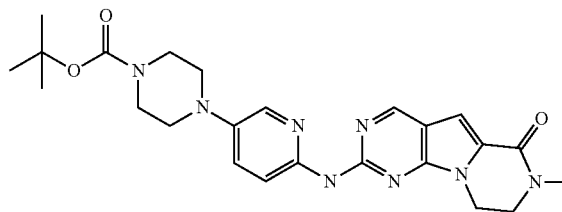
Compound 4
