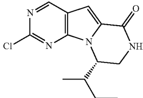
tert-butyl N-[(2S)-2-[(5-bromo-2-chloro-pyrimidin-4-yl)amino]-3-methyl-pentyl]carbamate
