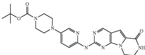
Compound 2
