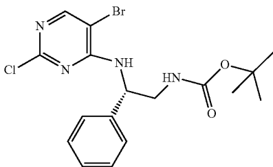
tert-butyl N-[(2S)-2-[(5-bromo-2-chloro-pyrimidin-4-yl)amino]-2-phenyl-ethyl] carbamate
