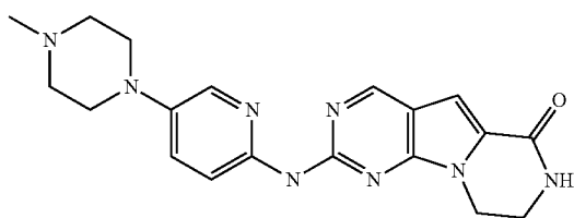
Compound 1
