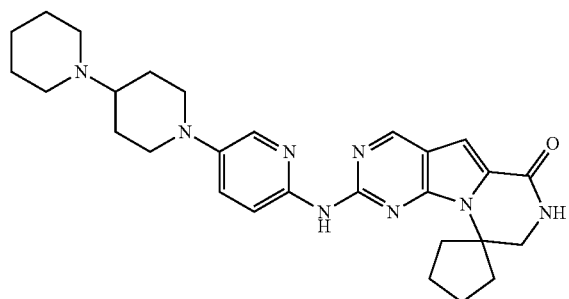
Compound 40
