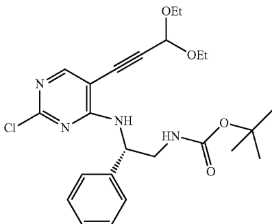
tert-butyl N-[(2S)-2-[[2-chloro-5-(3,3-diethoxyprop-1-ynyl)pyrimidin-4-yl]amino]-2-phenyl-ethyl]carbamate
