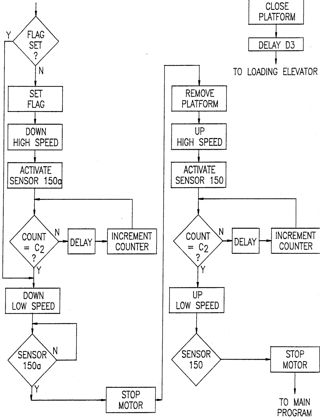
Fig. 2j LOADING ELEVATOR
