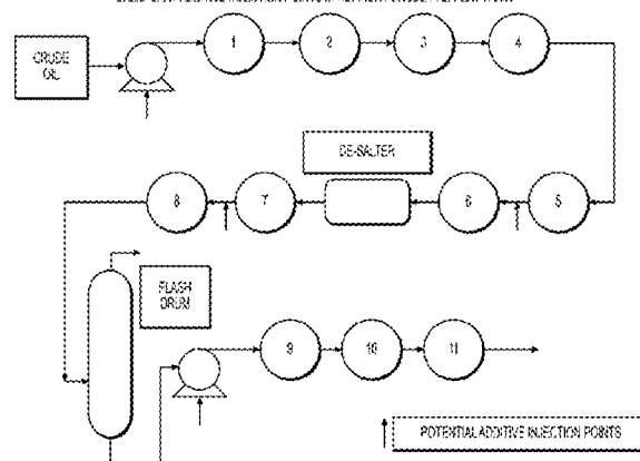
EXEMPLARY ADDITIVE INJECTION POINTS IN REFINERY CRUDE PRE-HEAT TRAIN
