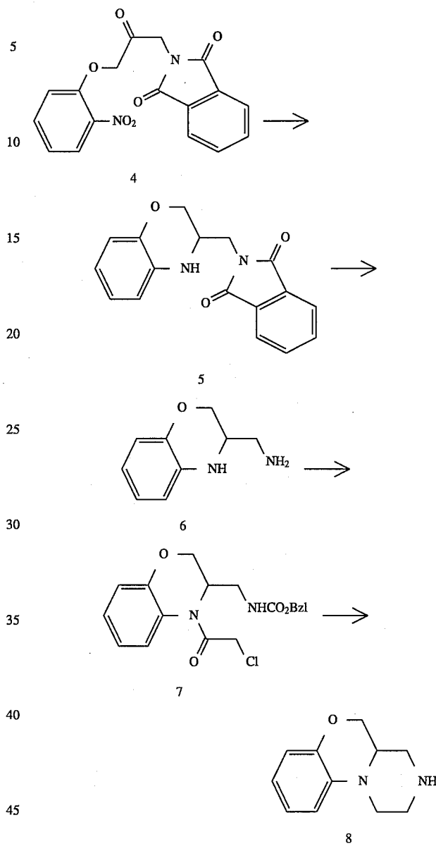
Reaction Scheme 2
