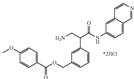
3-(3-amino-1-(isoquinolin-6-ylamino)-1-oxopropan-2-yl)benzyl 4-methoxybenzoate
