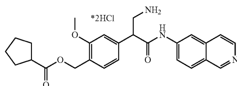
4-(3-amino-1-(isoquinolin-6-ylamino)-1-oxopropan-2-yl)-2-methoxybenzyl cyclopentanecarboxylate
