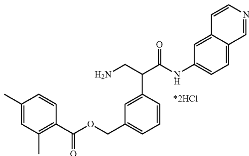
3-(3-amino-1-(isoquinolin-6-ylamino)-1-oxopropan-2-yl)benzyl 2,4-dimethylbenzoate
