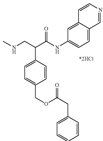
4-(1-(isoquinolin-6-ylamino)-3-(methylamino)-1-oxopropan-2-yl)benzyl 2-phenylacetate
