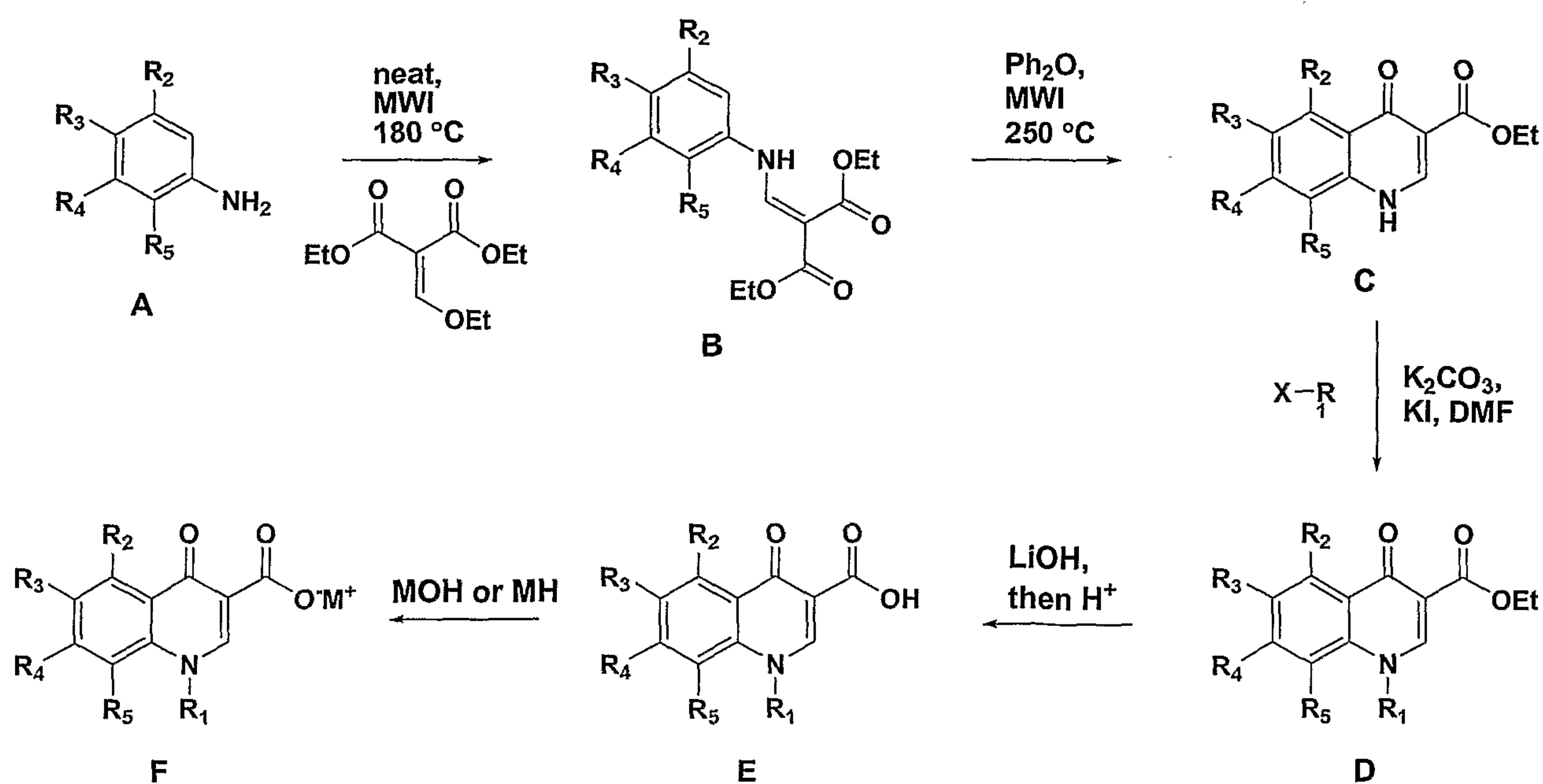
Scheme 1
