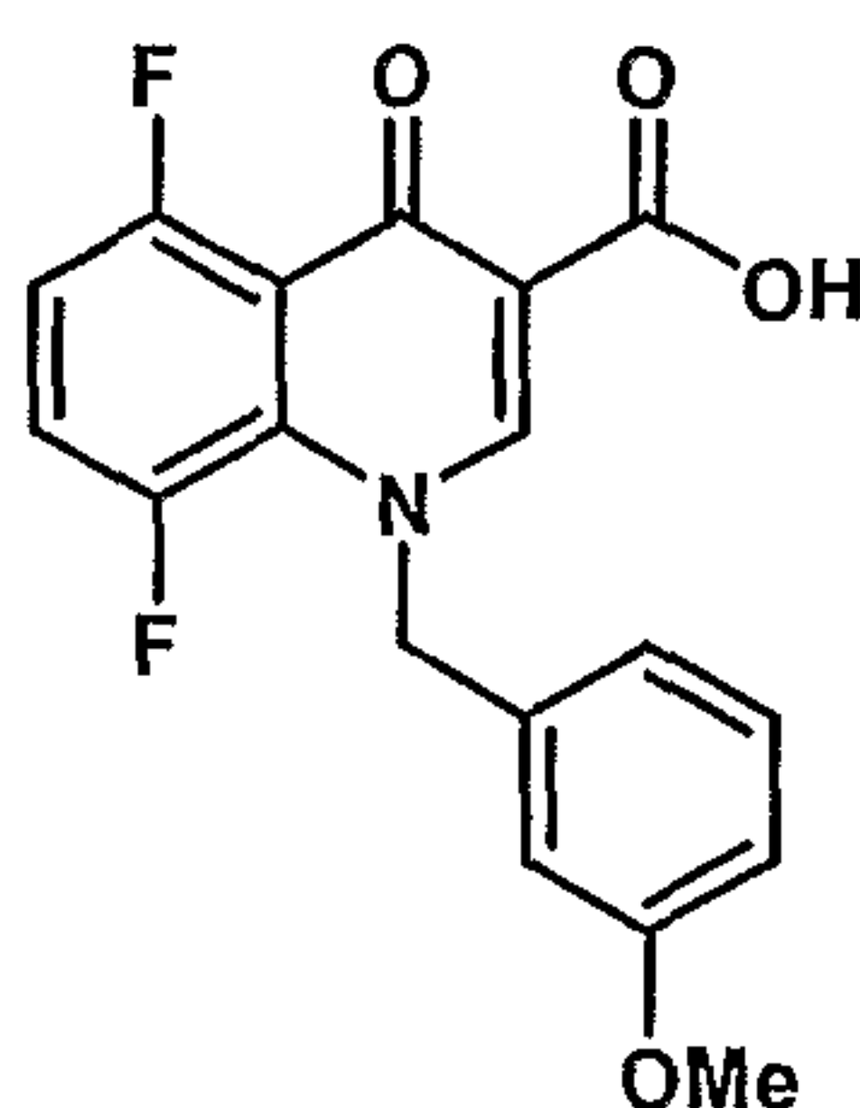
5,8-difluoro-1-(3-methoxybenzyl)-4-oxo-1,4-dihydroquinoline-3-carboxylic acid
