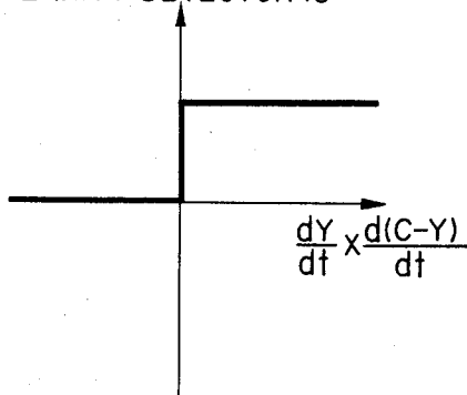
OUTPUT OF STEP POLARITY DETECTOR 15
