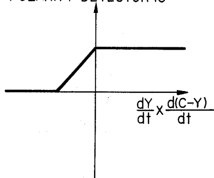
OUTPUT OF STEP POLARITY DETECTOR 15
