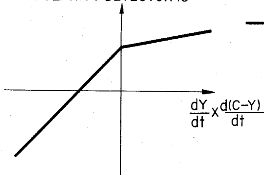
OUTPUT OF STEP POLARITY DETECTOR 15
