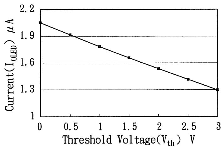
FIG. 2A(PRIOR ART)
