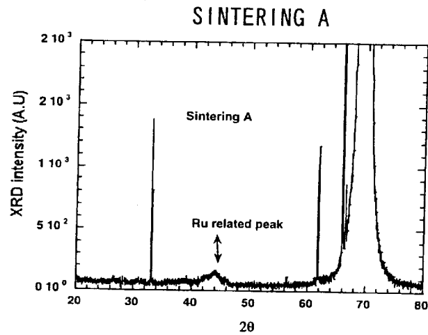
FIG. 9 (Prior Art)
