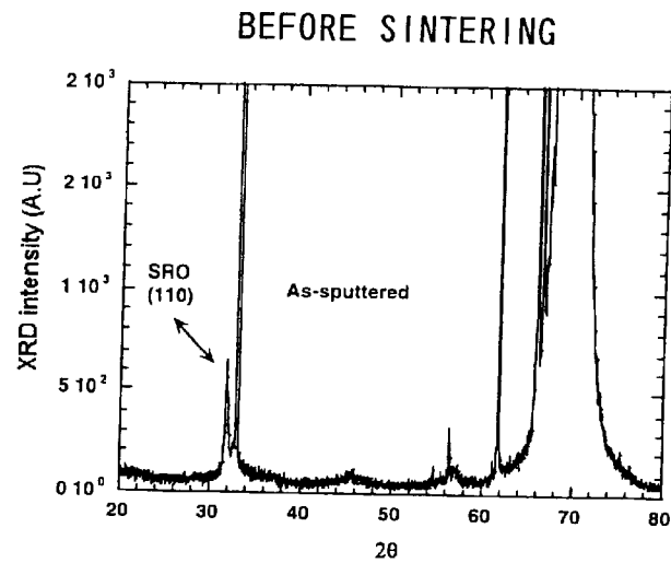
FIG. 9 (Prior Art)
