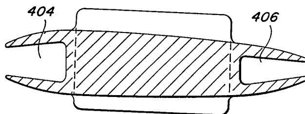
SECT S-S (B10)
