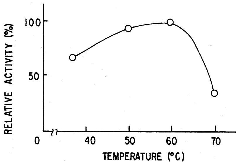
FIG 3 OPTIMUM TEMPERATURE
