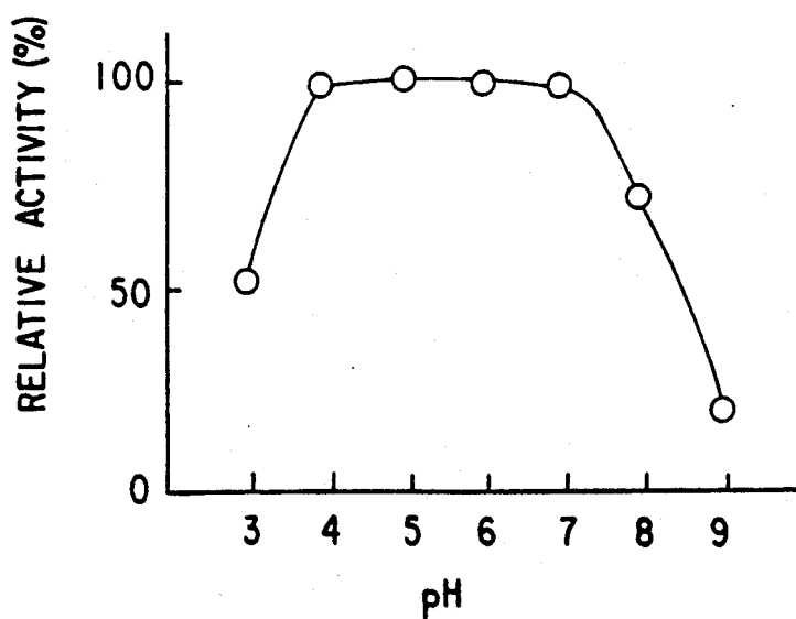
FIG 2 pH STABILITY
