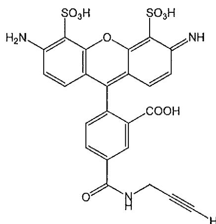
2-(6-amino-3-imino-4,5-disulfo-3H-xanthen-9-yl)-5-(prop-2-yn-1-ylcarbamoyl)benzoic acid
