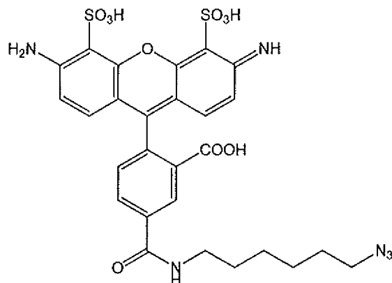
2-(6-amino-3-imino-4,5-disulfo-3H-xanthen-9-yl)-5-((6-azidohexyl)carbamoyl)benzoic acid
