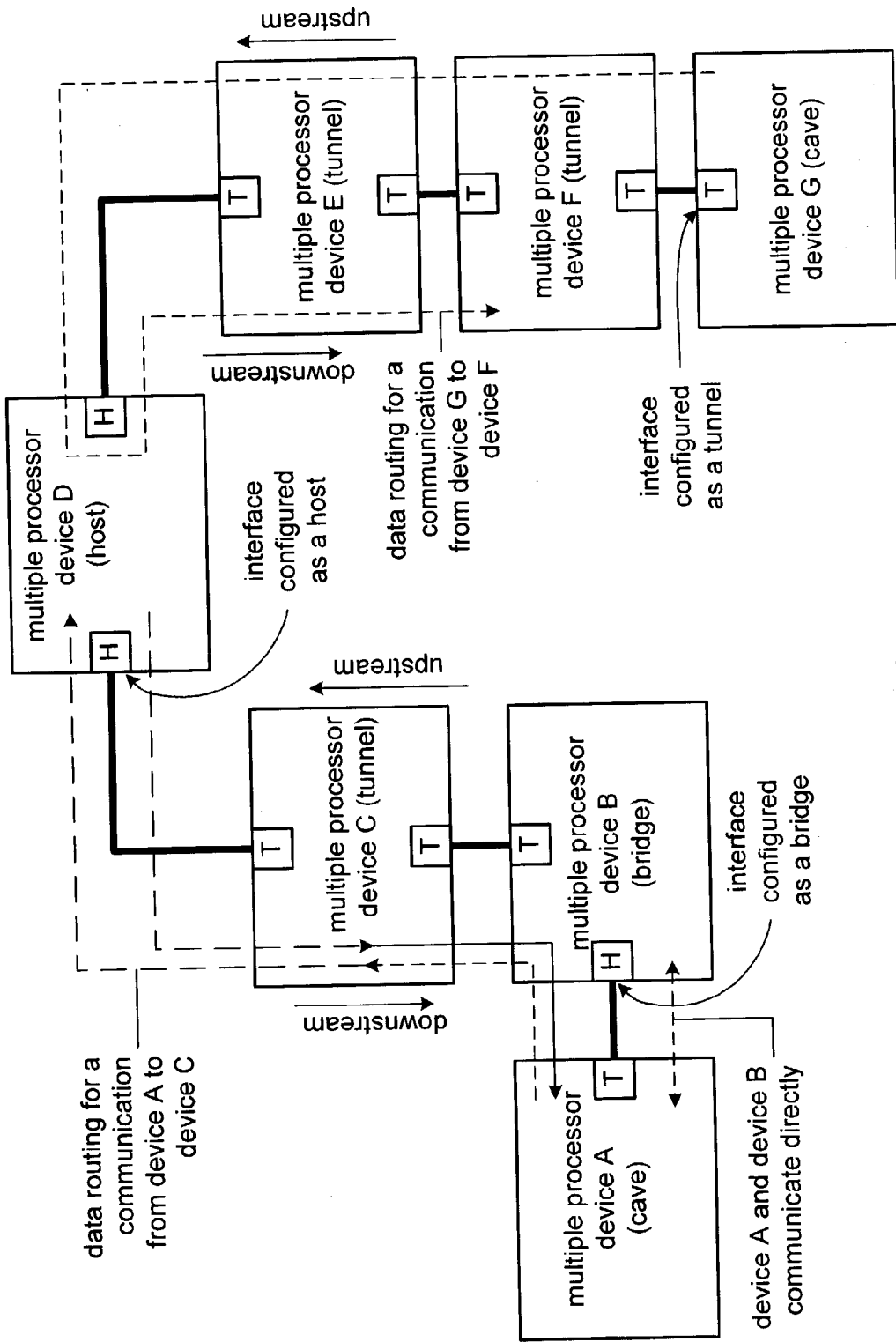
FIG. 1 processing system 10
