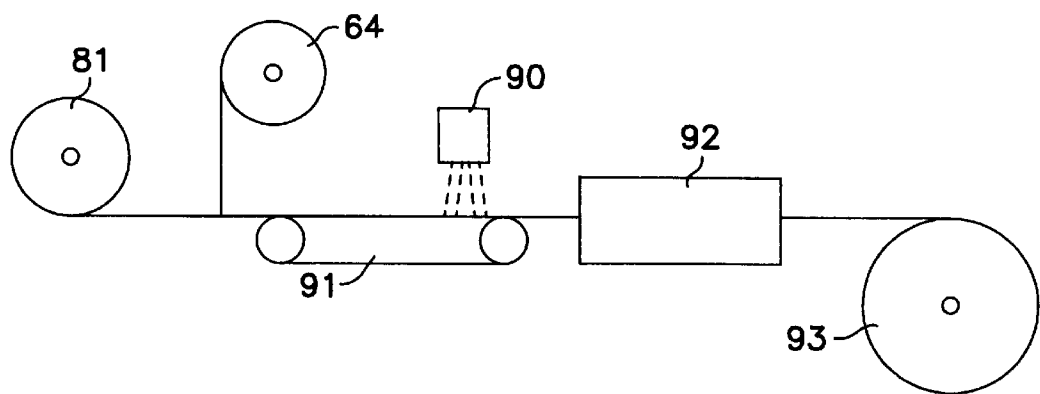
Typical Off-line Hydroentanglement process marrying a roll of nonwovens (long fiber) with a roll of paper (short fiber)
