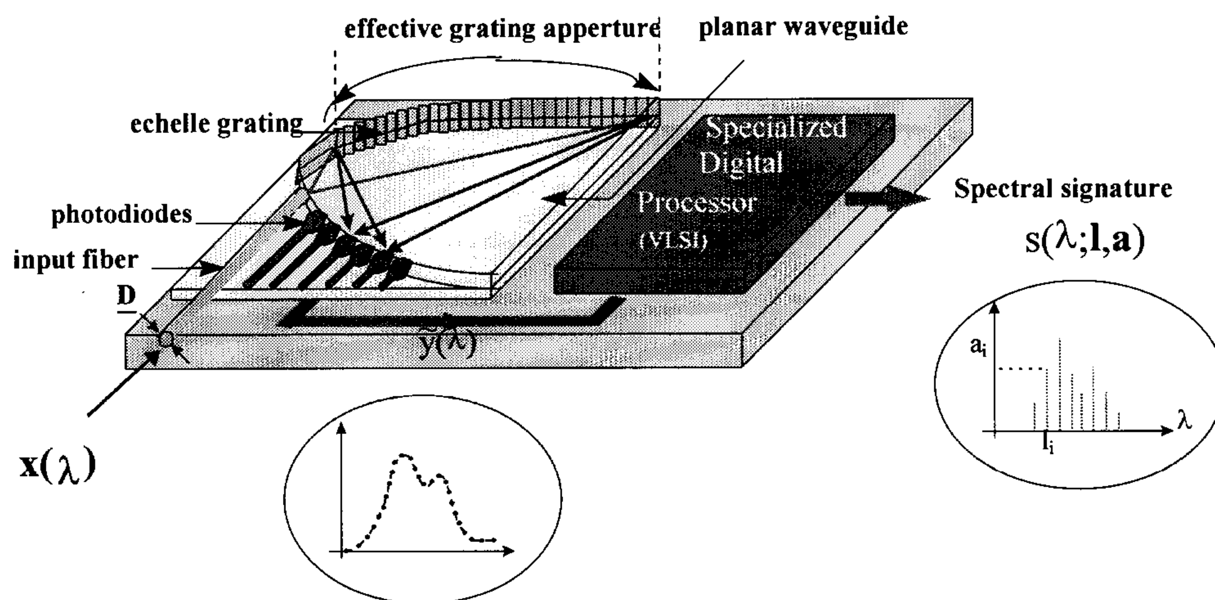
Fig. 8. Example of the hybrid, two-chip prototype, of the IISS/T;
