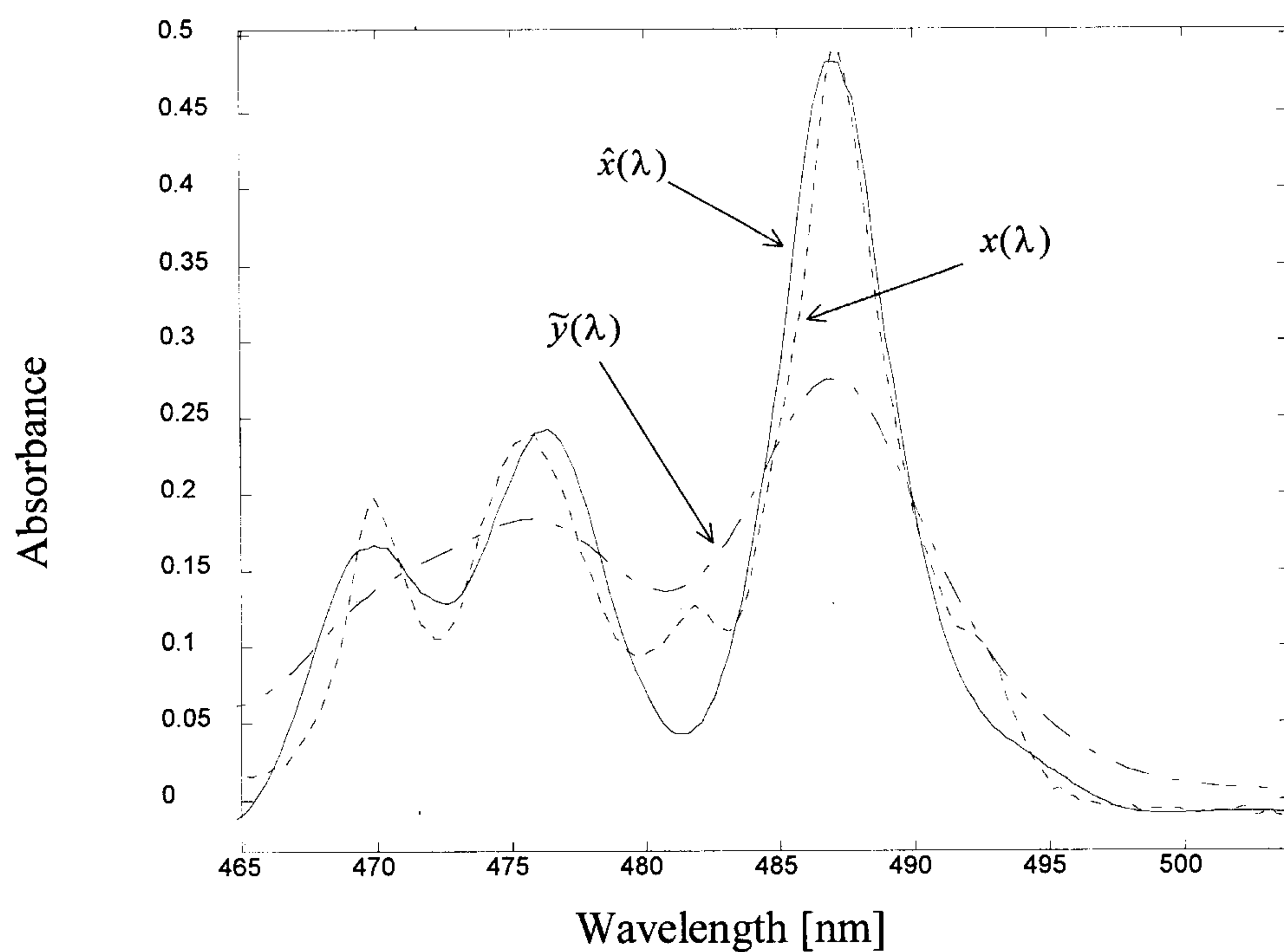
Fig.6 Effectiveness of the correction of the imperfections of the spectrometric transducer, by means of the specialized digital signal processor,
