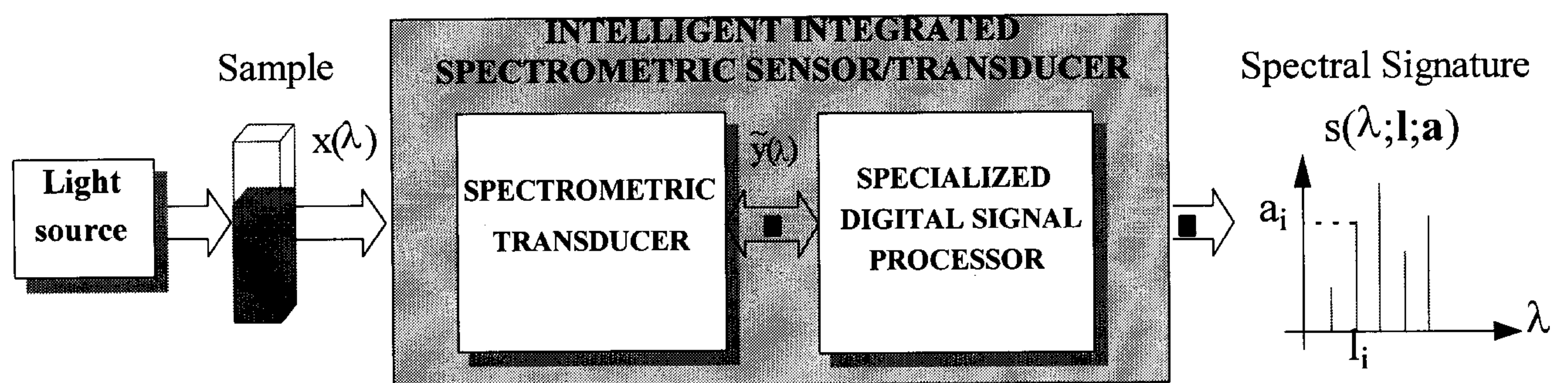
Fig 3. Measurement principle underlying the proposed intelligent spectrometric sensor /transducer (IISST);
