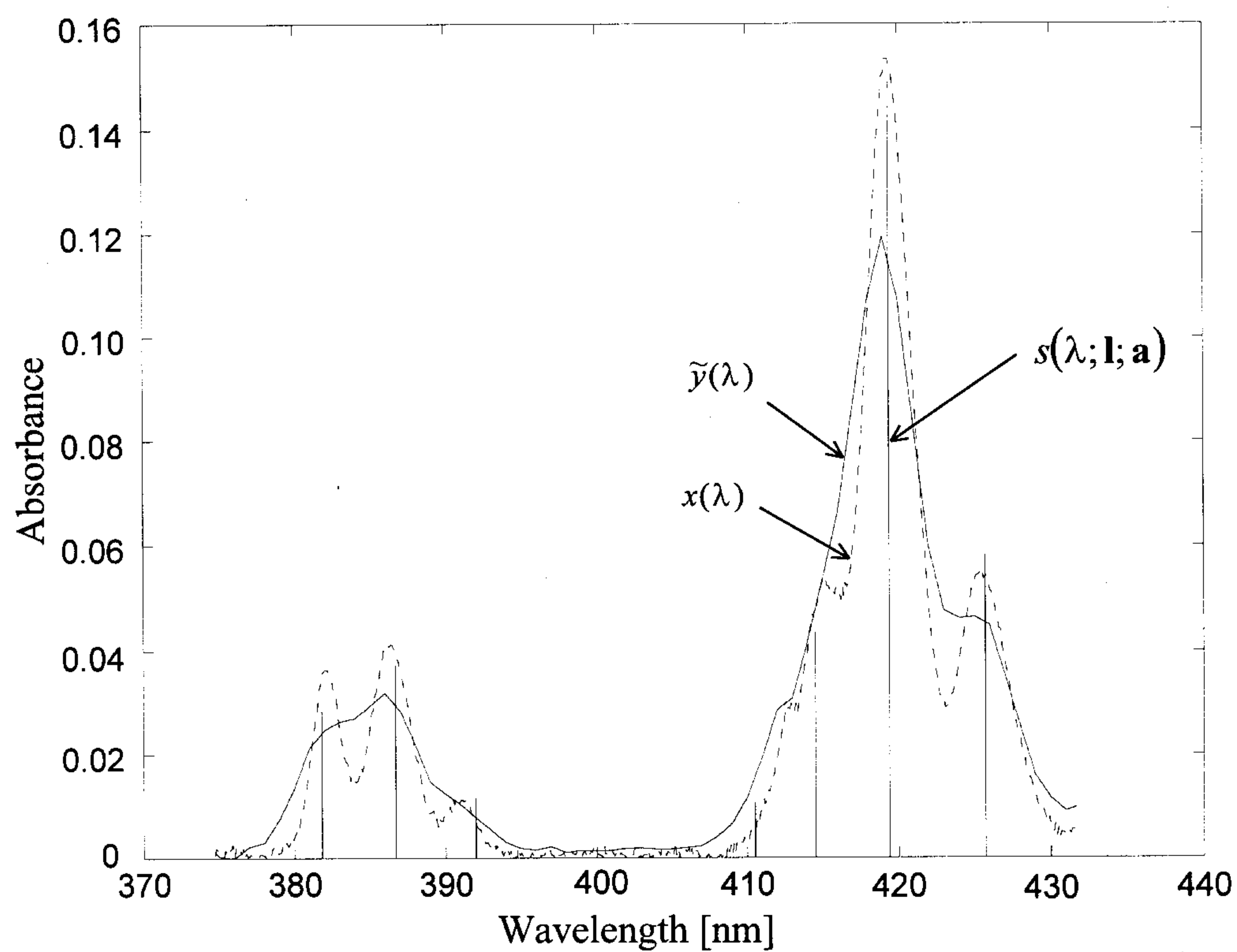
Fig 7 Results of the consecutive stages of signal processing performed by the model of the IISS/T, according to the invention.
