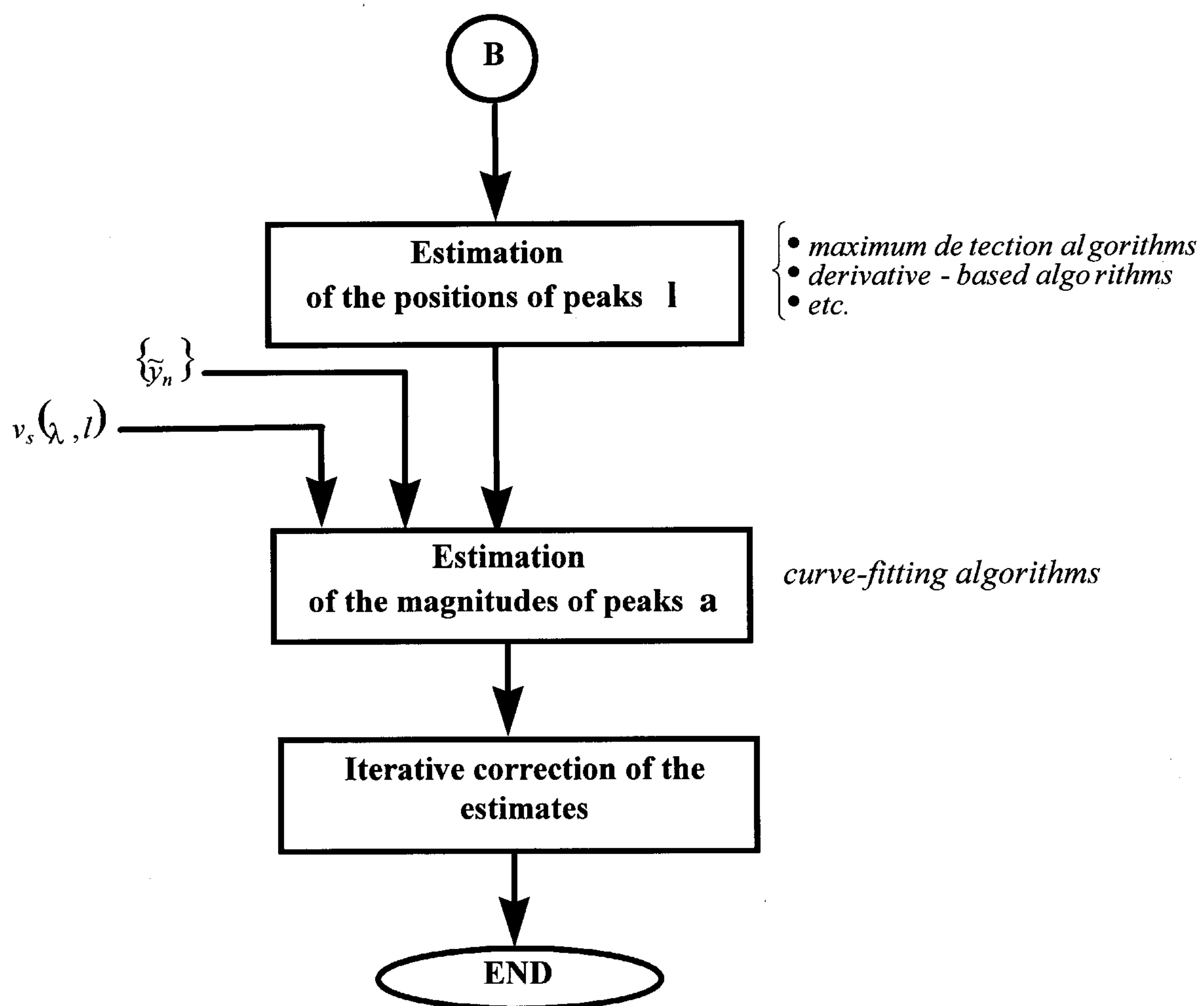
Fig. 11d The flow-diagram of the sub-procedure ISD_est.
