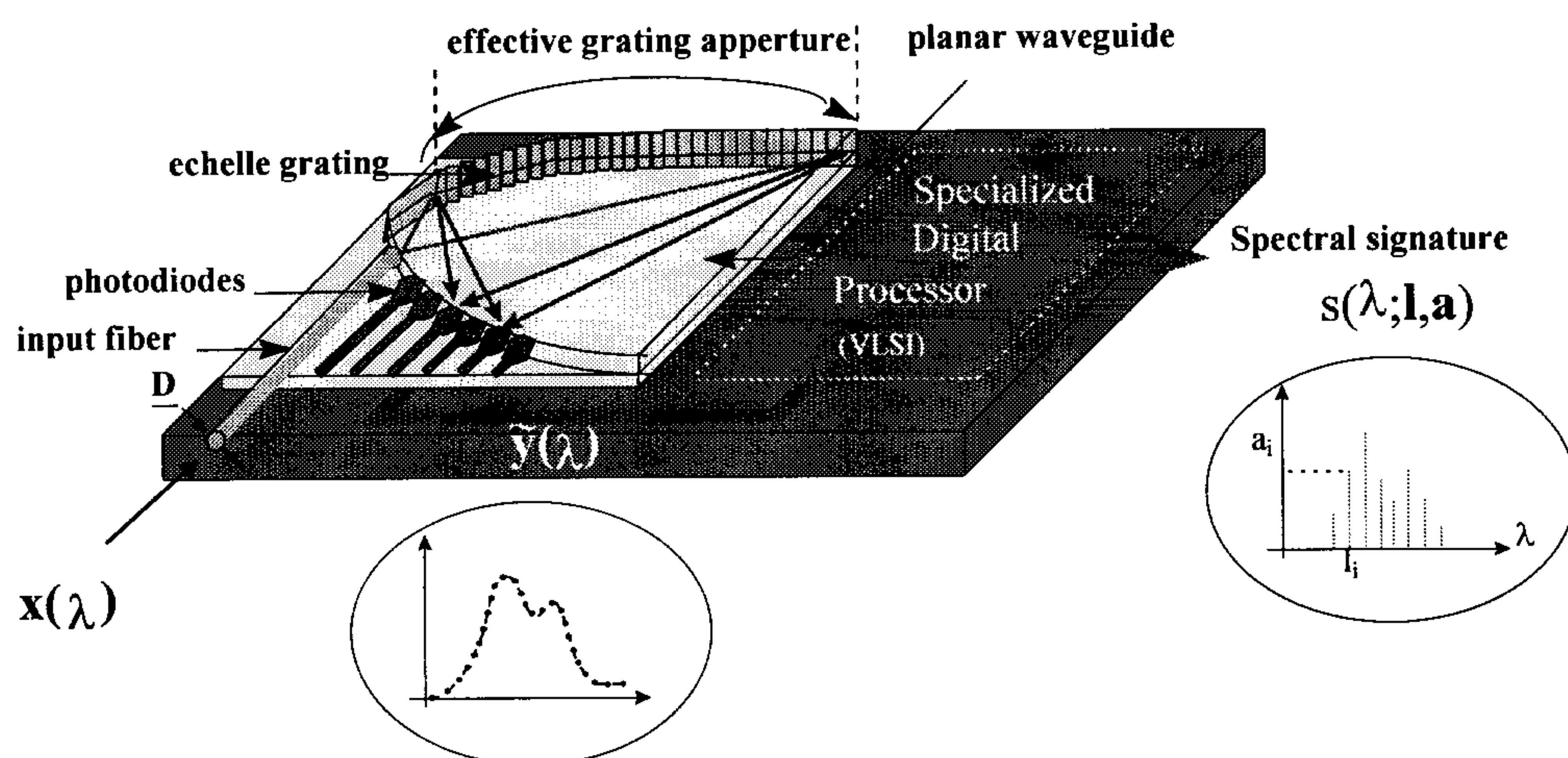
Fig. 5. Foreseen example of a generic structure of the IIS/T;
