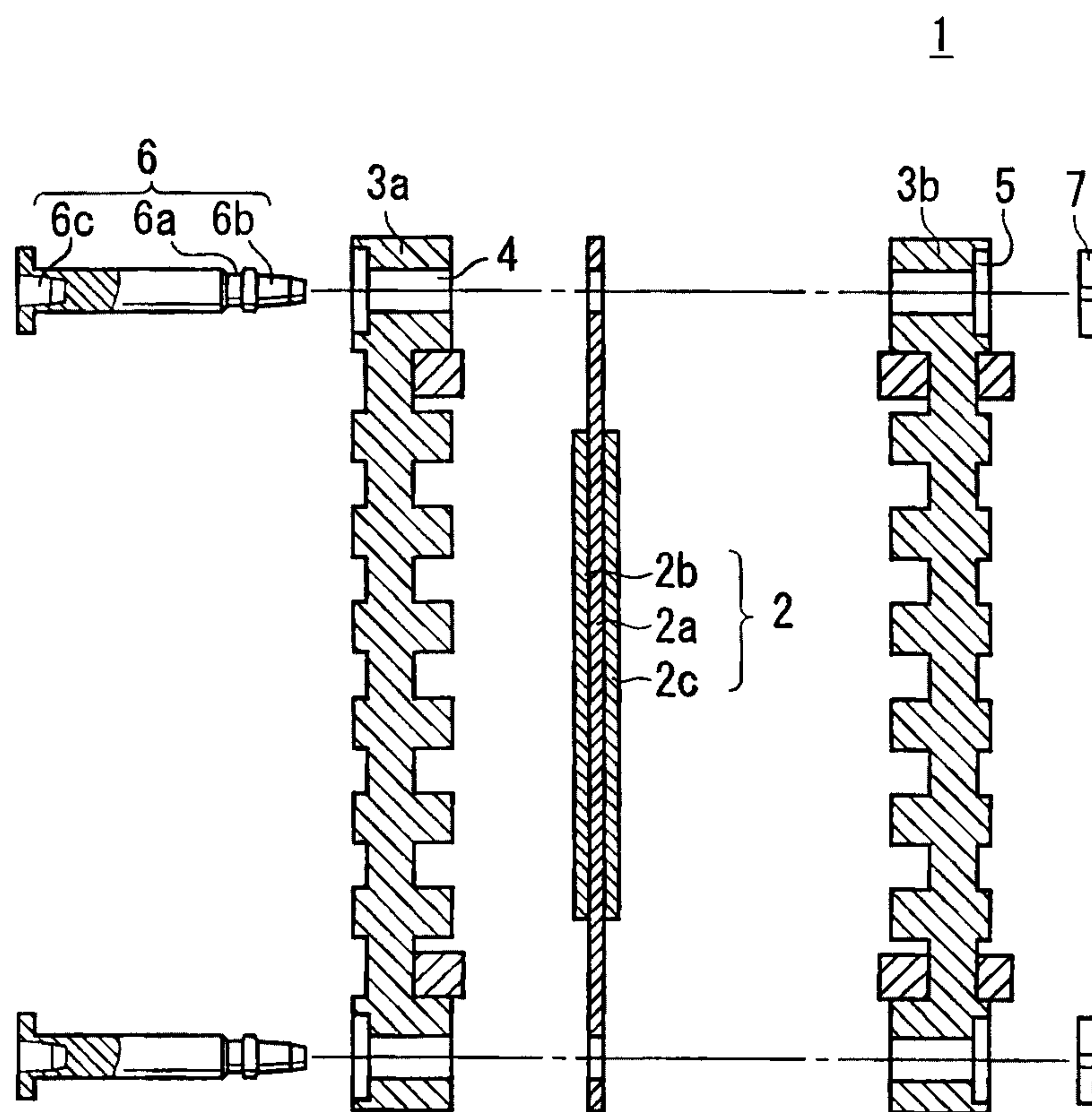
FIG. 9 Prior Art
