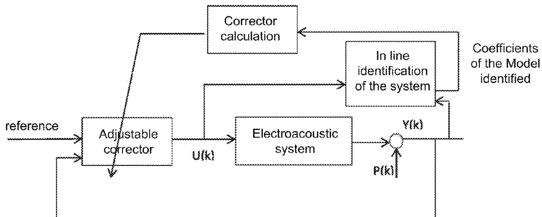
Fig.2: State of the art - indirect adaptive control
