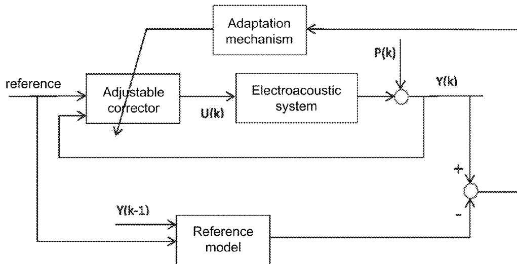
Fig.1: State of the art - direct adaptive control
