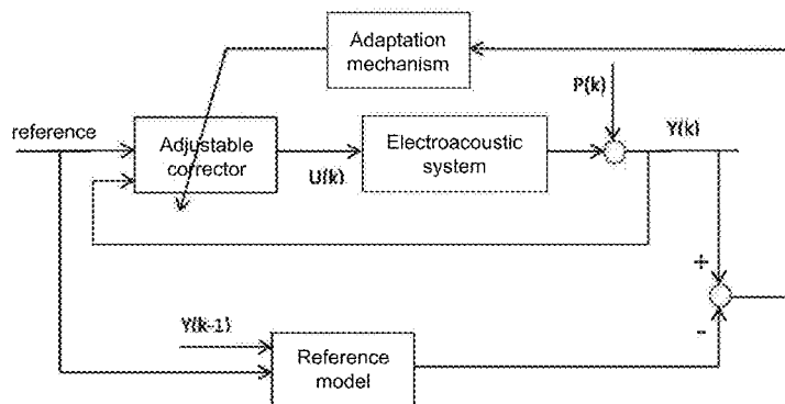
State of the art - direct adaptive control
