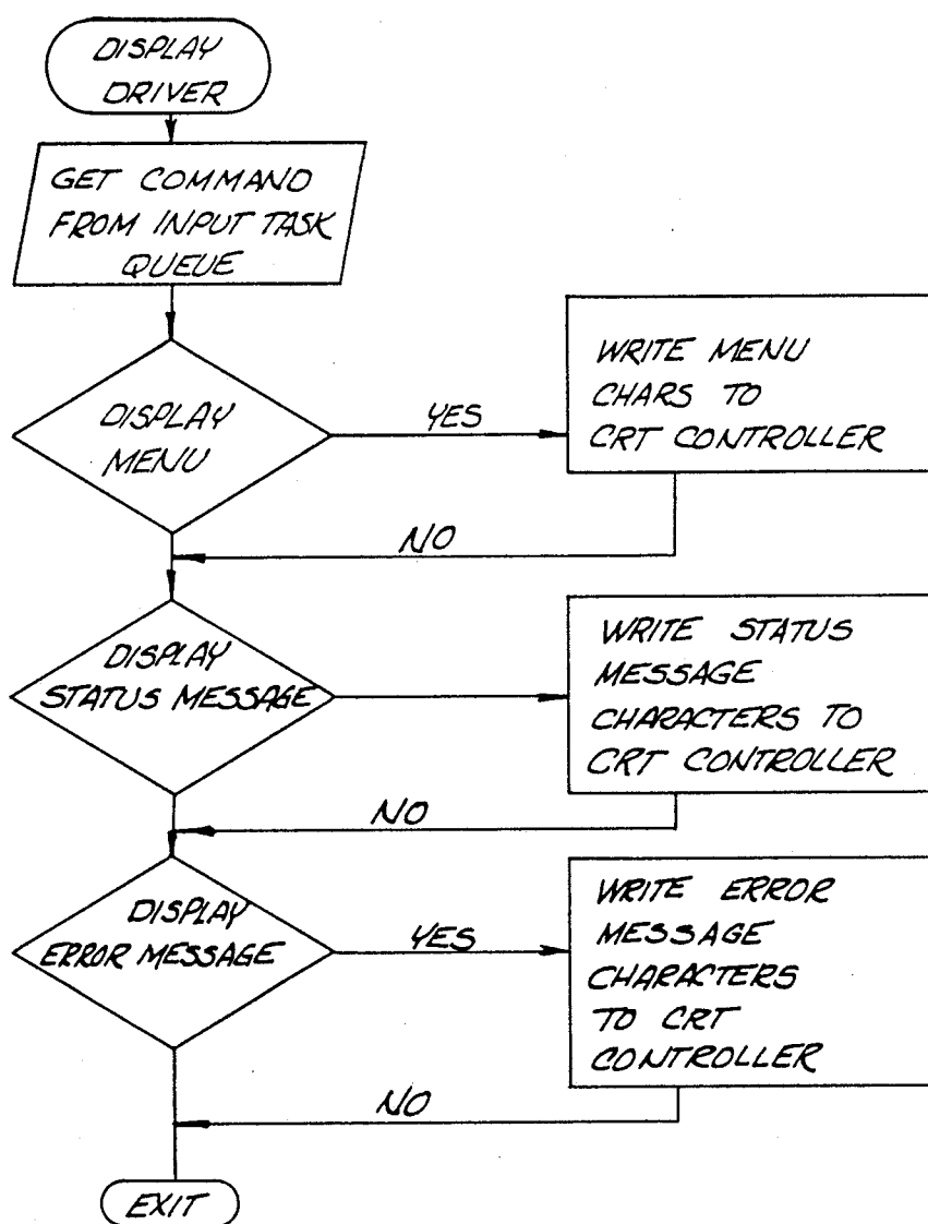
FIG. 14 CONSOLE MANAGER MODULE - DISPLAY DRIVER TASK
