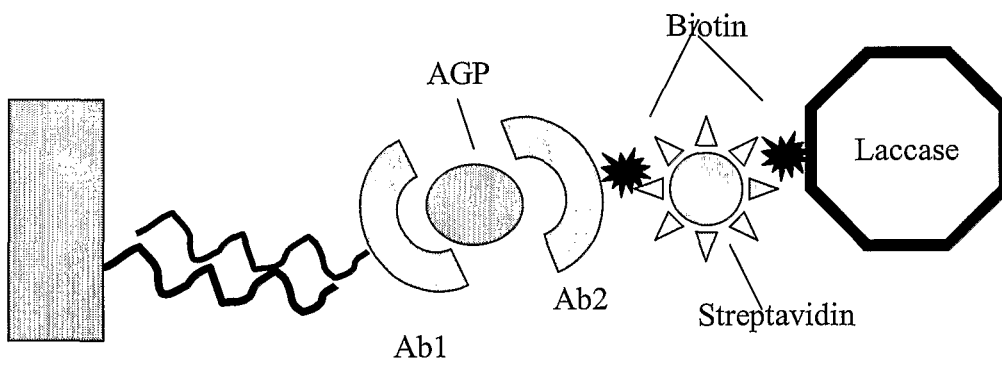
FIGURE 2 Laccase System
