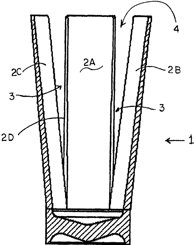
Figure 1 (Prior Art)
