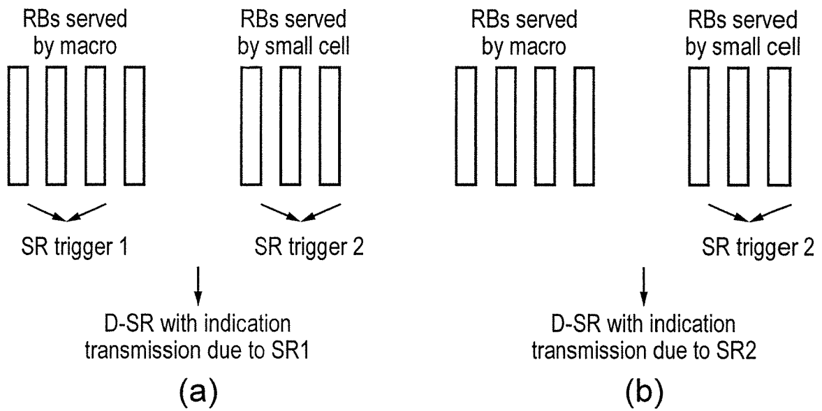
SR trigger and transmission of SR on D-SR when single D-SR is configured for the UE. (a) both SR1 and SR2 triggered at the same time and SR1 is transmitted on D-SR (b) both SR2 is triggered, SR2 is transmitted on D-SR
