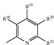
2-Pyridyl
