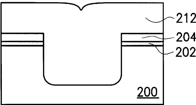
FIG. 2C (PRIOR ART)
