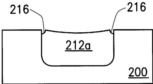
FIG. 2F (PRIOR ART)
