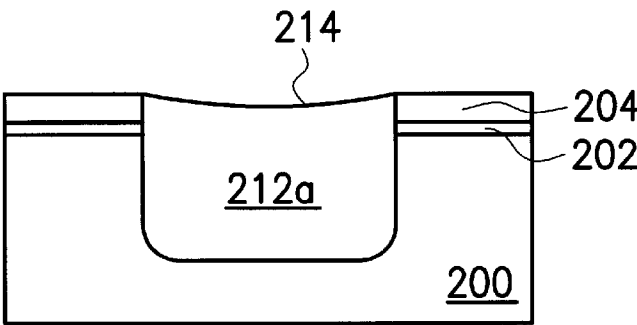
FIG. 2D (PRIOR ART)
