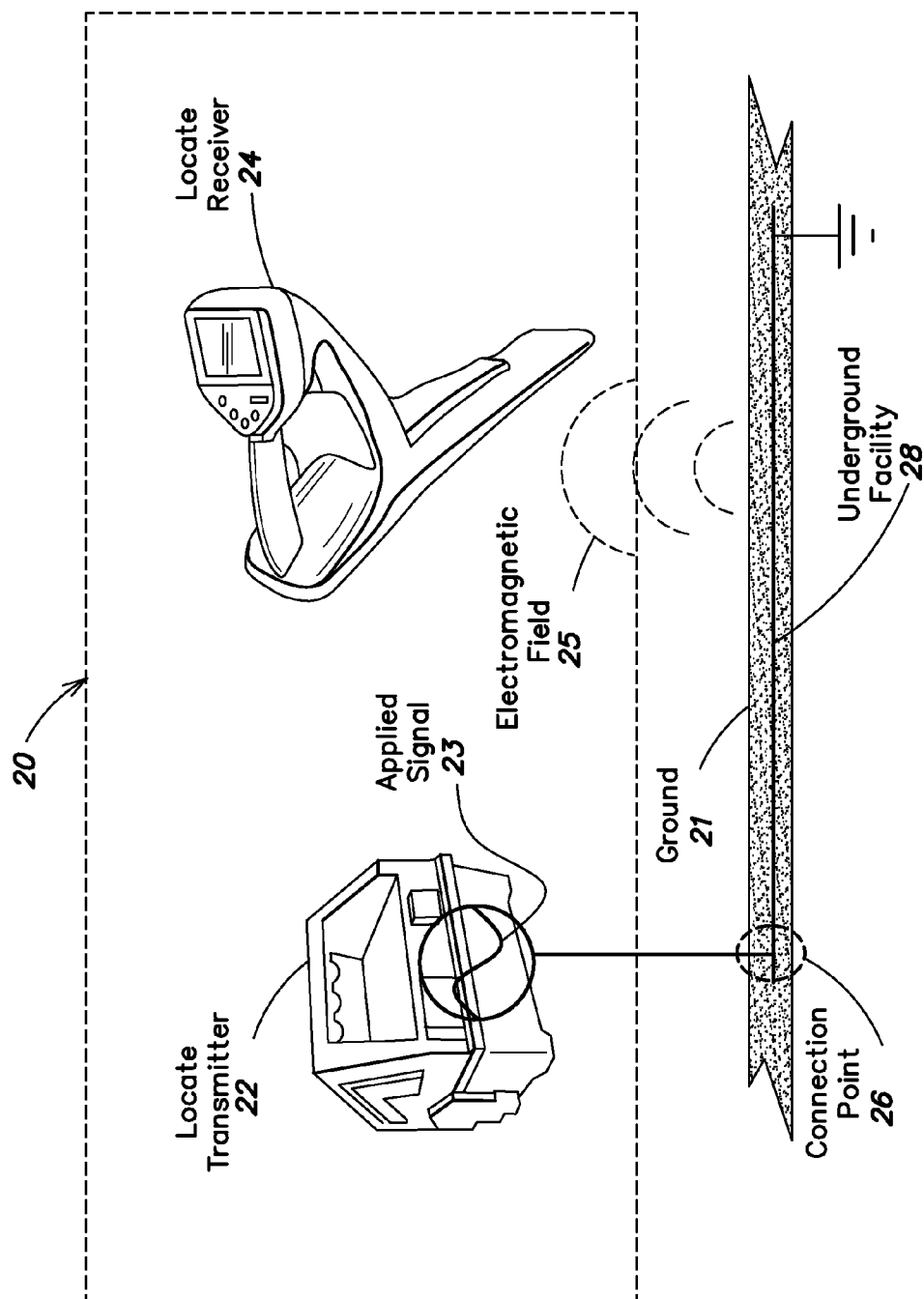
FIG. 2 (Prior Art)
