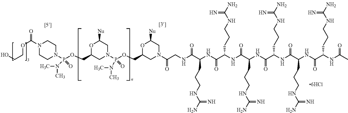
PPMOs 1-39
