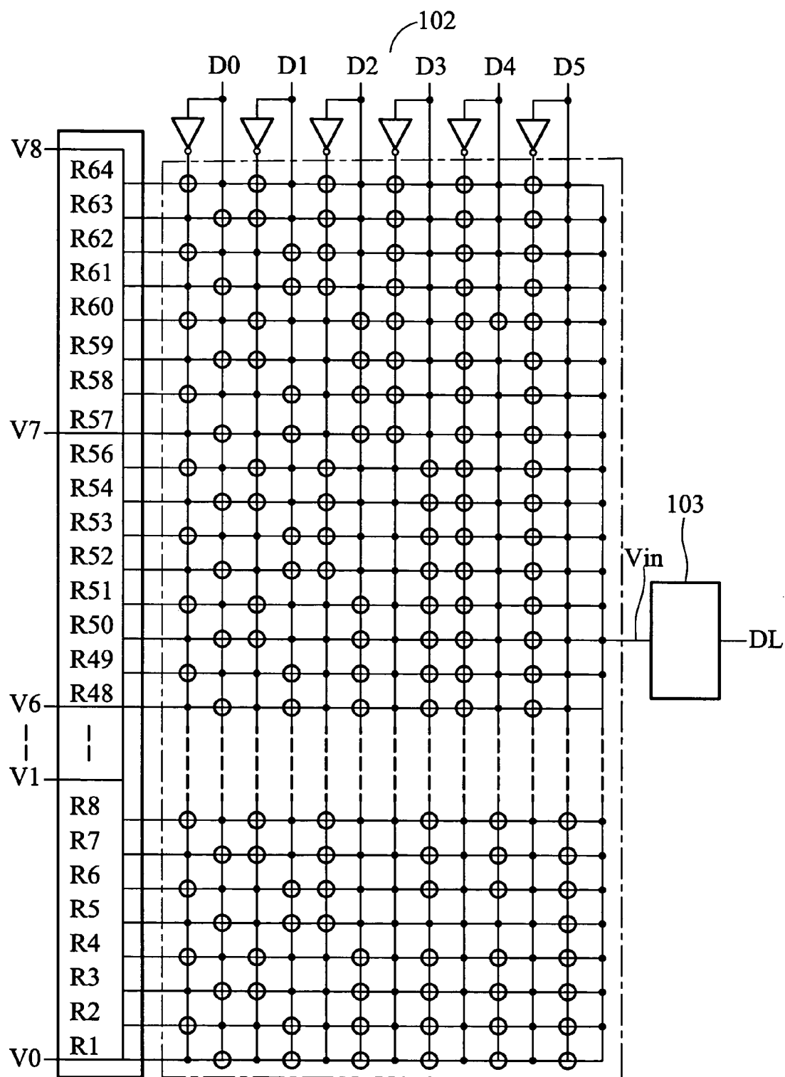
FIG. 1 ( RELATED ART )
