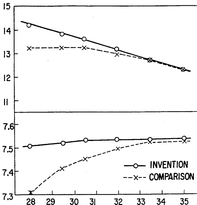
SINTERED DENSITY (g/cm 3 ) Nd+Dy (wt%)
