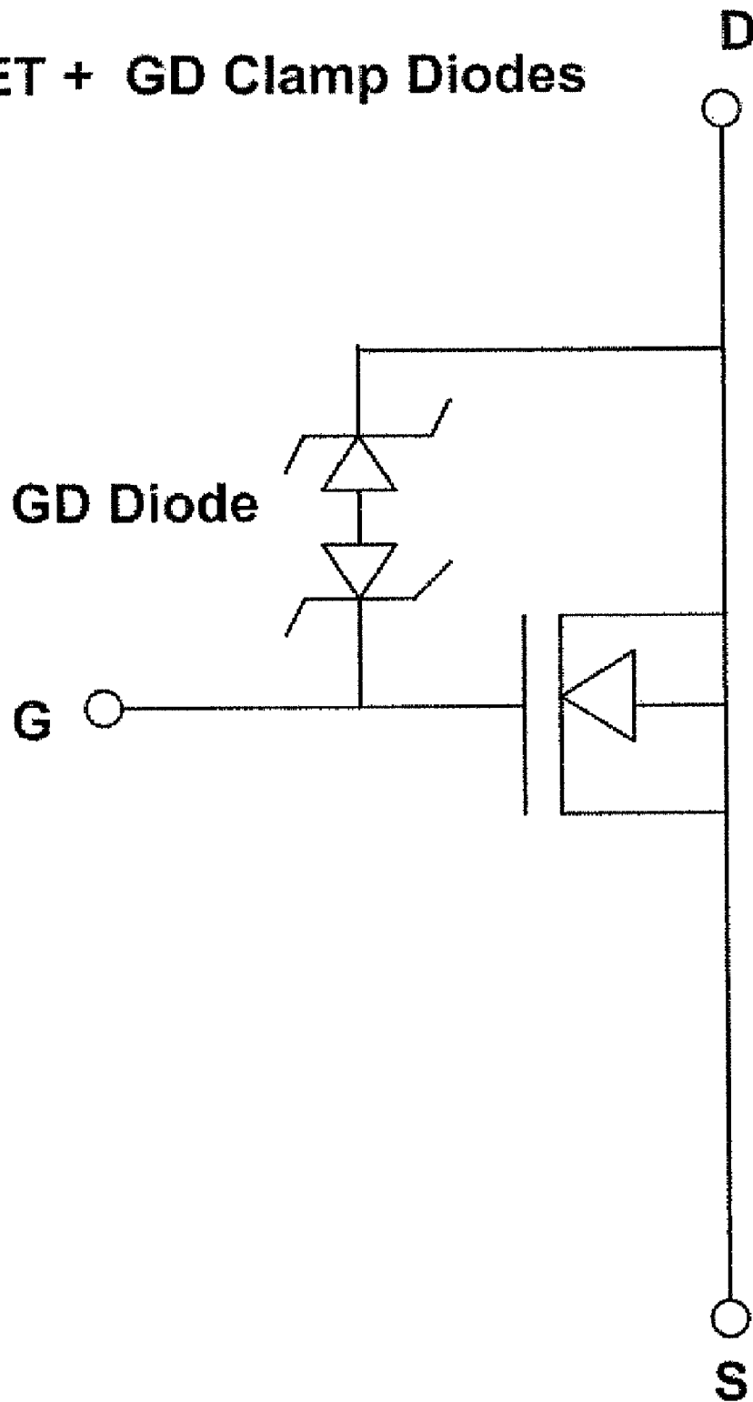
Fig.1 (Pior Art)
