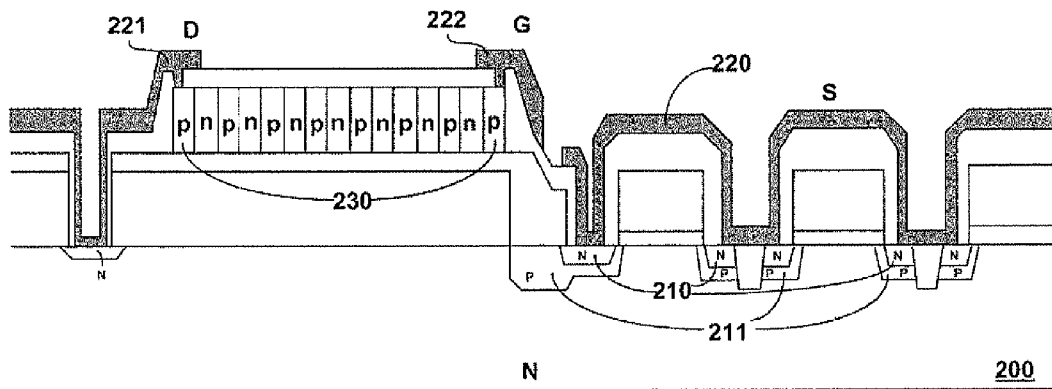
Fig.2 (Pior Art)
