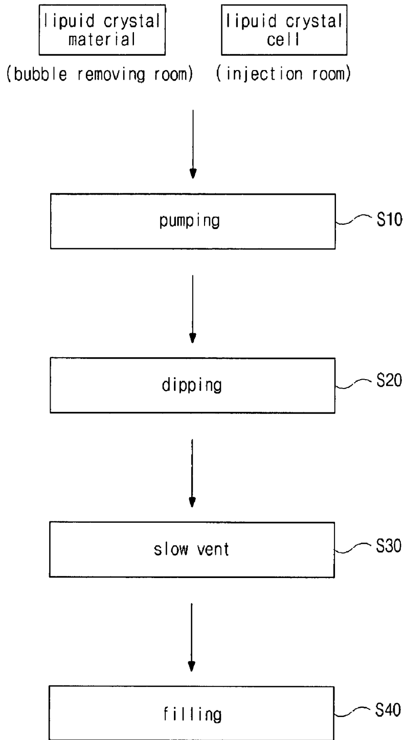
FIG. 3 RELATED ART
