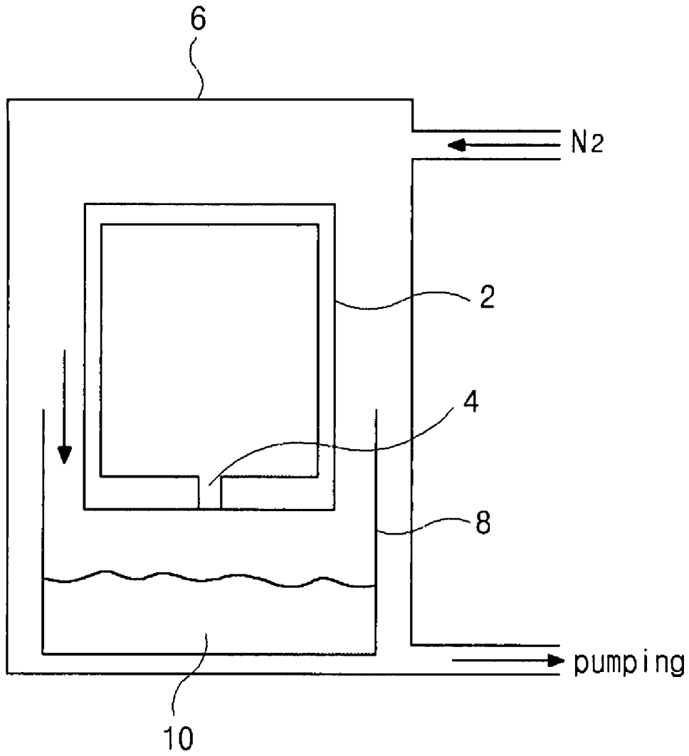
FIG. 2 RELATED ART
