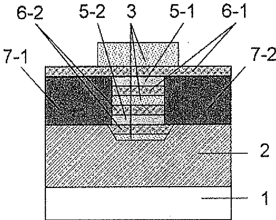
B-B' Cross-sectional View
