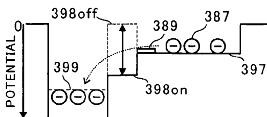
FIG. 7C PRIOR ART
