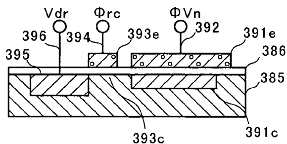
FIG. 7C PRIOR ART
