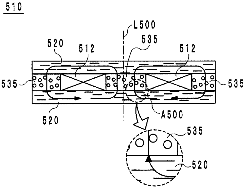
FIG. 21 PRIOR ART
