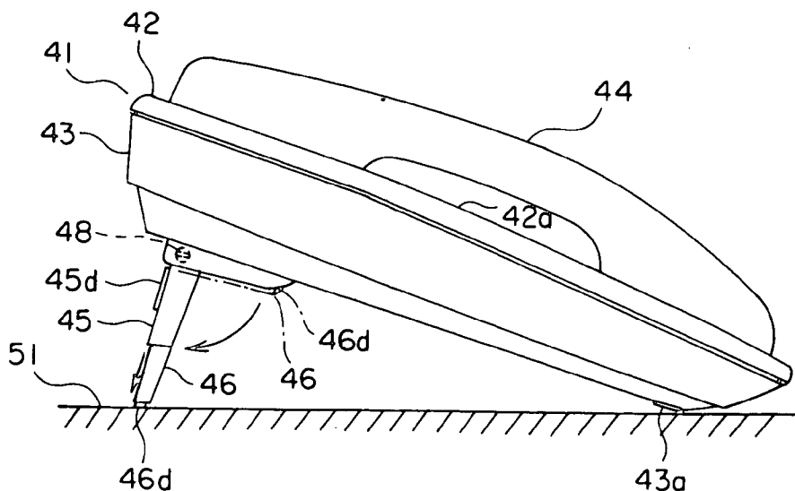
FIG. 11 PRIOR ART
