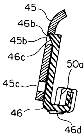
FIG. 8 PRIOR ART
