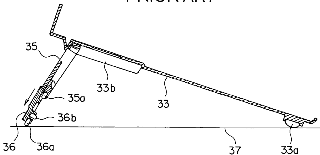
FIG. 5 PRIOR ART
