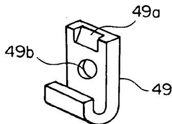
FIG. 7 PRIOR ART
