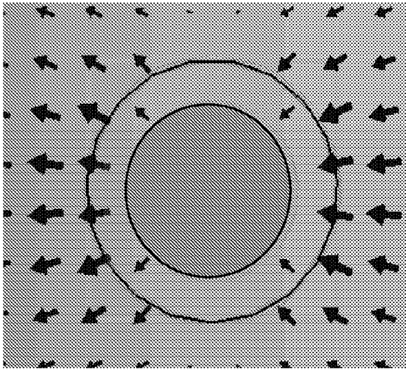
Hybrid mode (HE 11 ) 2168
