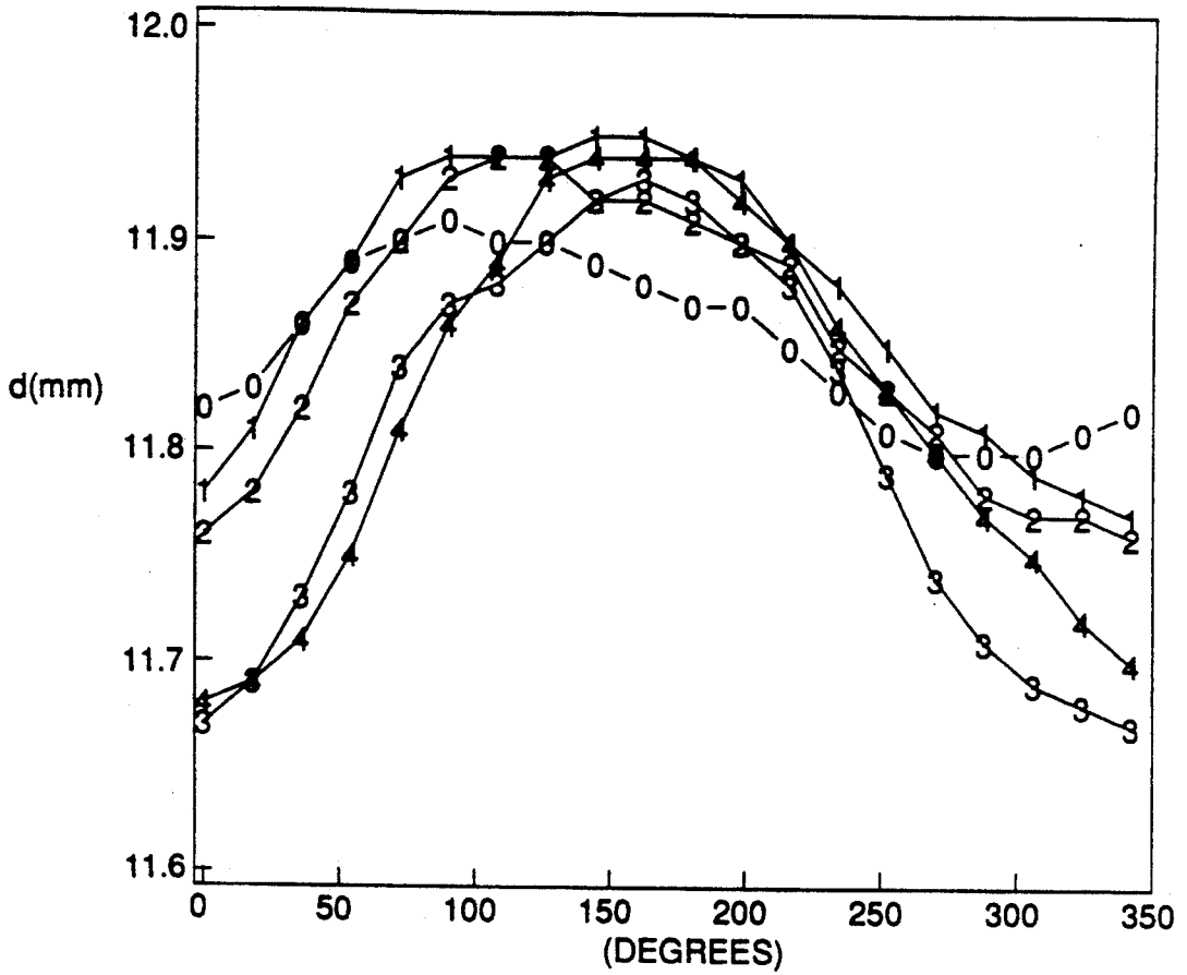
ECCENTRICITY PROFILE (BEFORE ETCHING)
