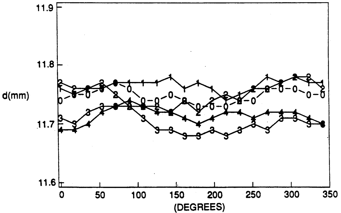
ECCENTRICITY PROFILE (AFTER ETCHING)
