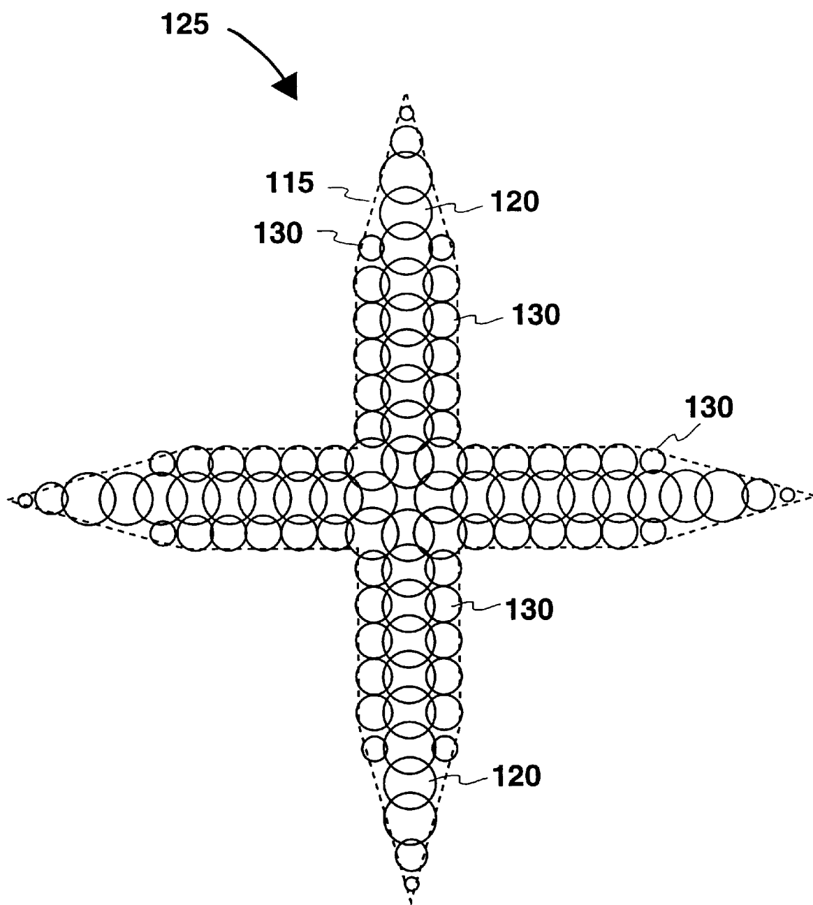
FIG. 4 (PRIOR ART)
