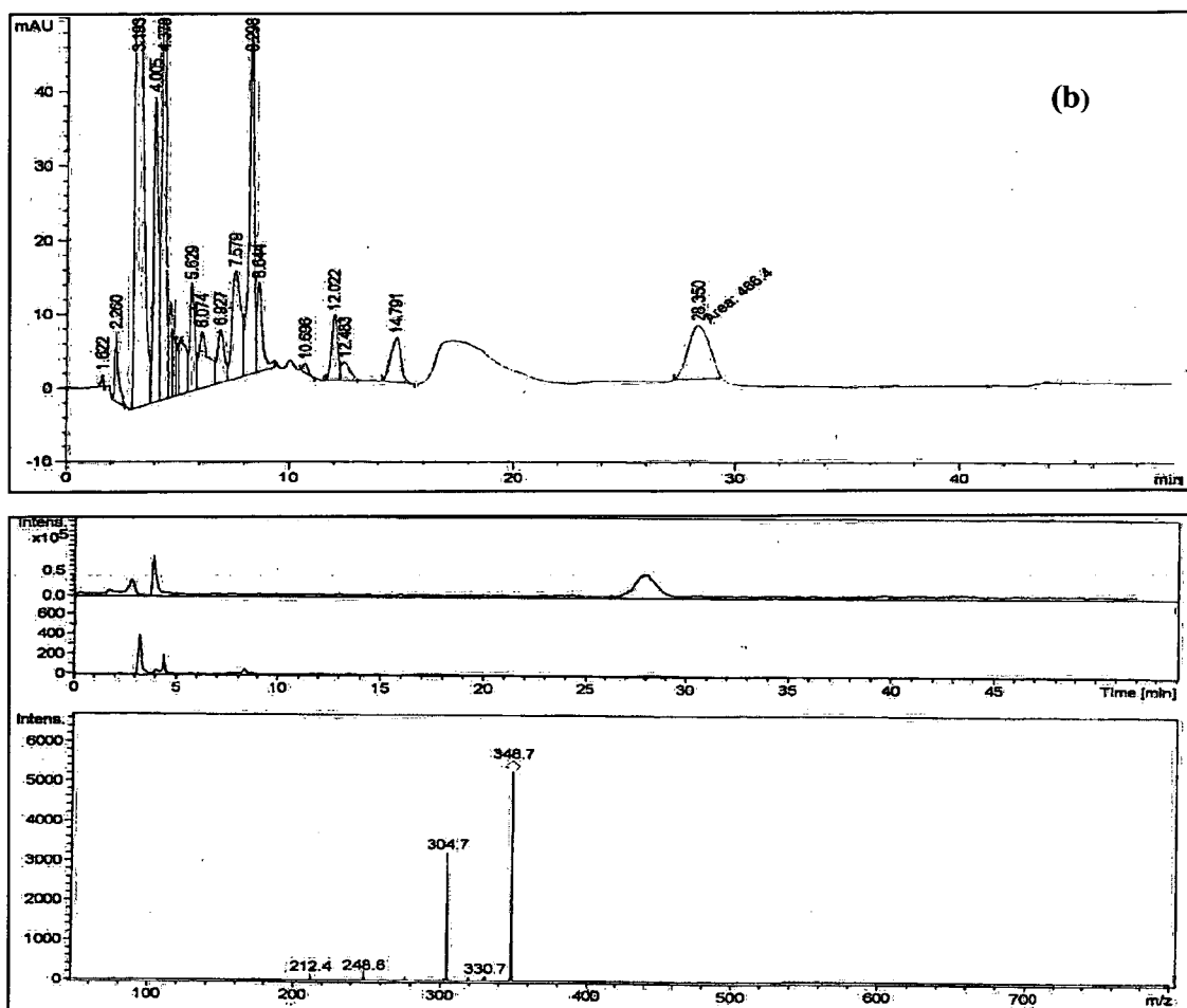
Fig.3: (b) Fungal Camptothecin
