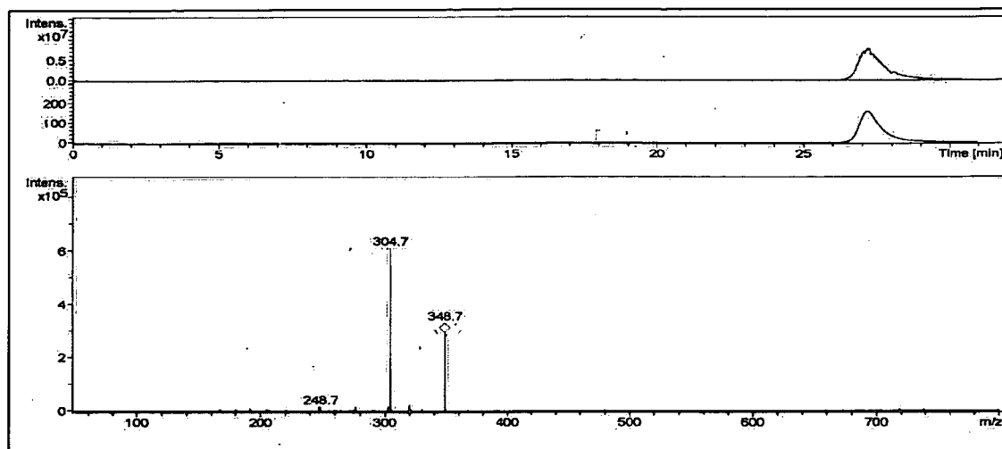
Fig.3: (a) LC/MS profile of Authentic
