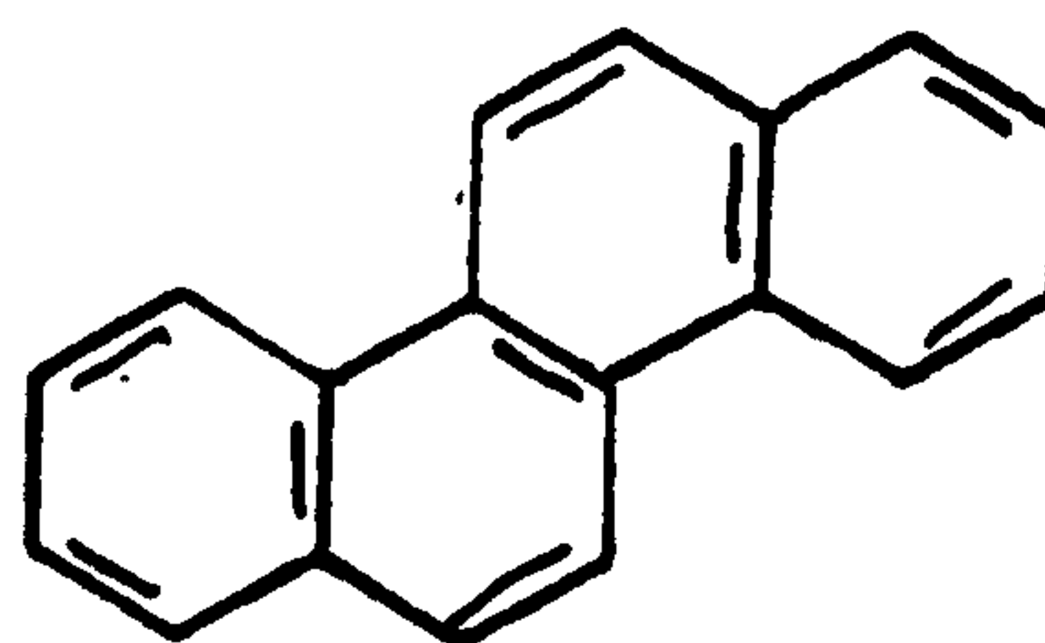
CHRYSENE
