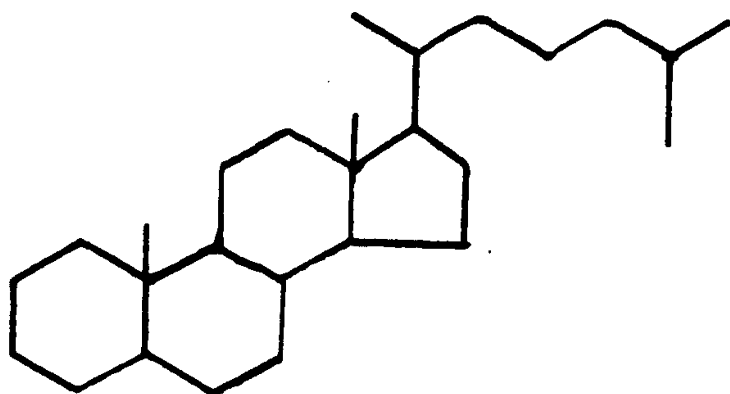
CHOLESTANE
