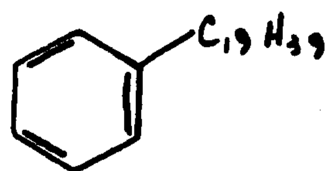
NONADECYLBENZENE
