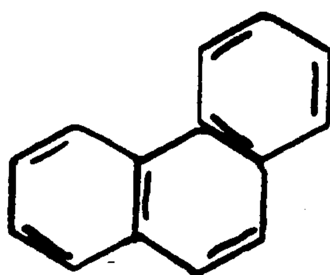
PHENANTHRENE
