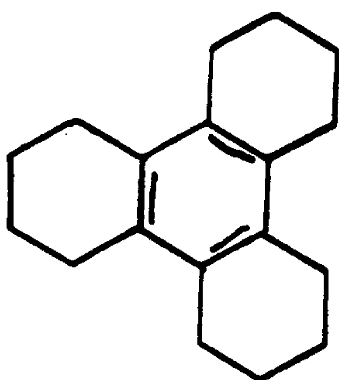
DODECAHYDROTRIPHEylene
