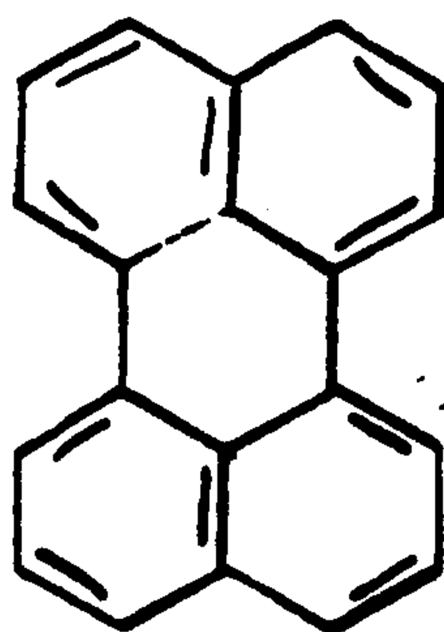
PERYLENE
