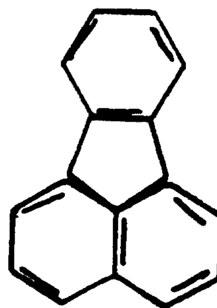
FLUORANTHENE
