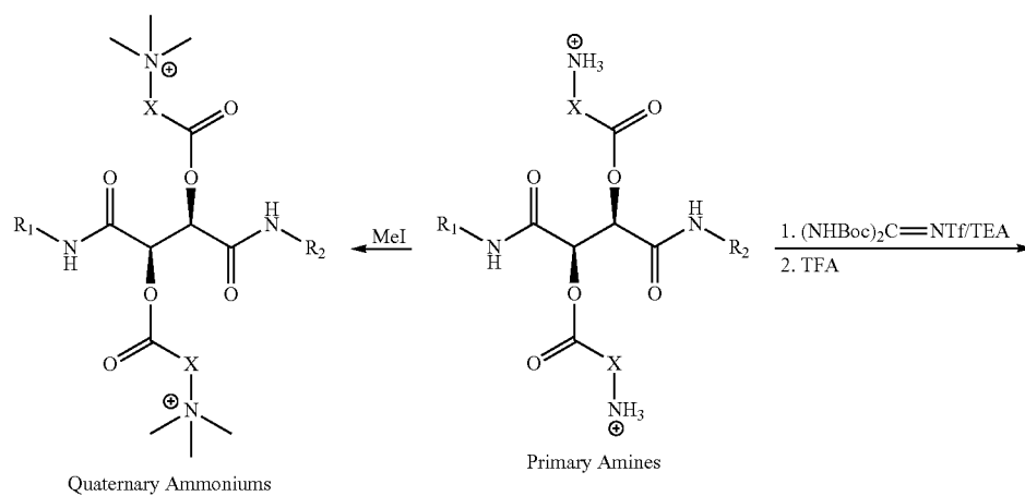
Scheme 4: Generation of Certain Amine Moieties
