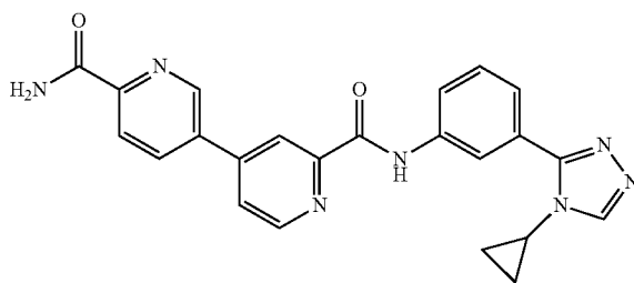
N2'-(3-(4-cyclopropyl-4H-1,2,4-triazol-3-yl)phenyl)- 3,4'-bipyridine-2',6-dicarboxamide
