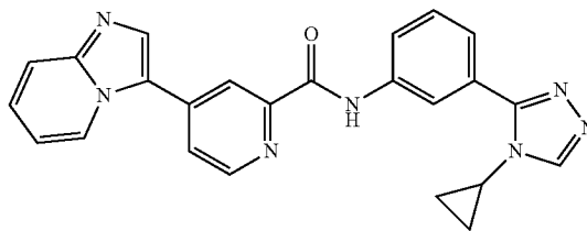
N-(3-(4-cyclopropyl-4H-1,2,4-triazol-3-yl)phenyl)-4-(imidazo[1,2-a]pyridin-3-yl)picolinamide
