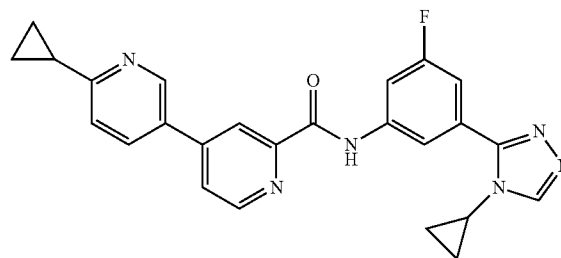
6-cyclopropyl-N-(3-(4-cyclopropyl-4H-1,2,4-triazol-3-yl)-5-fluorophenyl)-3,4'-bipyridine-2'-carboxamide
