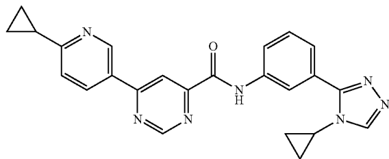
N-(3-(4-cyclopropyl-4H-1,2,4-triazol-3-yl)phenyl)-6-(6-cyclopropylpyridin-3-yl)pyrimidine-4-carboxamide
