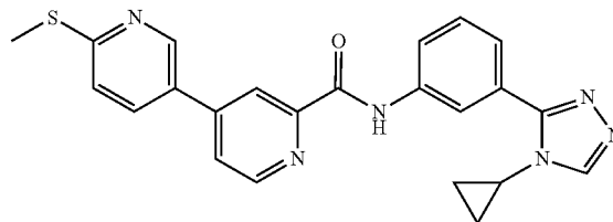
N-(3-(4-cyclopropyl-4H-1,2,4-triazol-3-yl)phenyl)-6-(methylthio)-3,4'-bipyridine-2'-carboxamide
