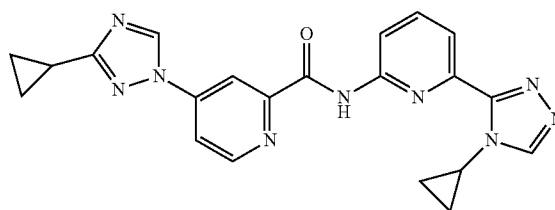
4-(3-cyclopropyl-1H-1,2,4-triazol-1-yl)-N-(6-(4-cyclopropyl-4H-1,2,4-triazol-3-yl)pyridin-2-yl)picolinamide
