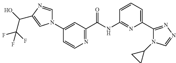
N-(6-(4-cyclopropyl-4H-1,2,4-triazol-3-yl)pyridin-2-yl)-4-(4-(2,2,2-trifluoro-1-hydroxyethyl)-1H-imidazol-1-yl)picolinamide
