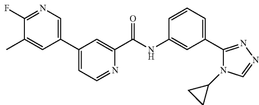
N-(3-(4-cyclopropyl-4H-1,2,4-triazol-3-yl)phenyl)- 6-fluoro-5-methyl-3,4'-bipyridine-2'-carboxamide
