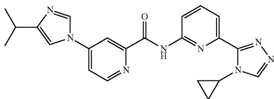
N-(6-(4-cyclopropyl-4H-1,2,4-triazol-3-yl)pyridin-2-yl)-4-(4-isopropyl-1H-imidazol-1-yl)picolinamide
