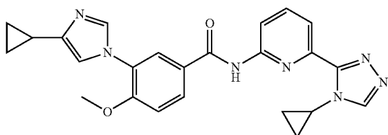
3-(4-cyclopropyl-1H-imidazol-1-yl)-N-(6-(4-cyclopropyl-4H-1,2,4-triazol-3-yl)pyridin-2-yl)-4-methoxybenzamide
