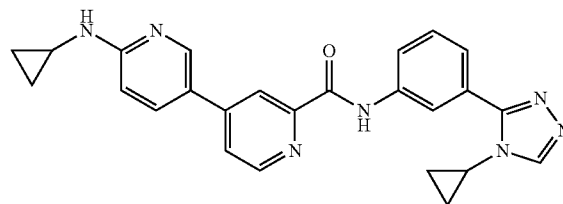
N-(3-(4-cyclopropyl-4H-1,2,4-triazol-3-yl)phenyl)-6-(cyclopropylamino)-3,4'-bipyridine-2'-carboxamide
