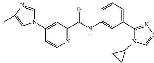
N-(3-(4-cyclopropyl-4H-1,2,4-triazol-3-yl)phenyl)-4-(1-methyl-1H-pyrazol-4-yl)picolinamide
