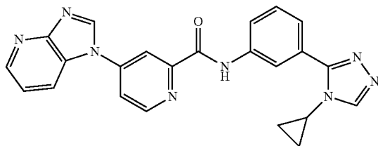
N-(3-(4-cyclopropyl-4H-1,2,4-triazol-3-yl)phenyl)-4-(1H-imidazo[4,5-b]pyridin-1-yl)picolinamide
