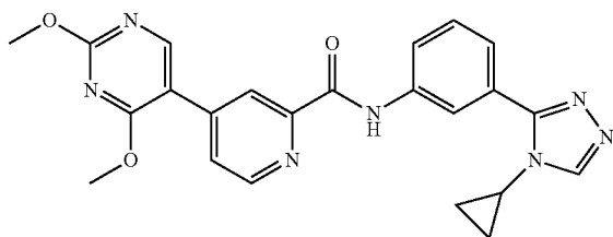
N-(3-(4-cyclopropyl-4H-1,2,4-triazol-3-yl)phenyl)- 4-(2,4-dimethoxy-5-yl)picolinamide
