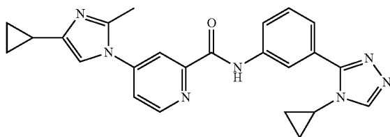
4-(4-cyclopropyl-2-methyl-1H-imidazol-1-yl)-N-(3-(4-cyclopropyl-4H-1,2,4-triazol-3-yl)phenyl)picolinamide
