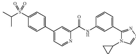
N-(3-(4-cyclopropyl-4H-1,2,4-triazol-3-yl)phenyl)- 4-(4-(isopropylsulfonyl)-phenyl)picolinamide
