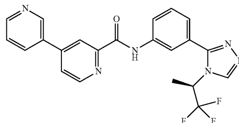
(R)-N-(3-(4-(1,1,1-trifluoropropan-2-yl)-4H-1,2,4-triazol-3-yl)phenyl)-3,4'-bipyridine-2'-carboxamide
