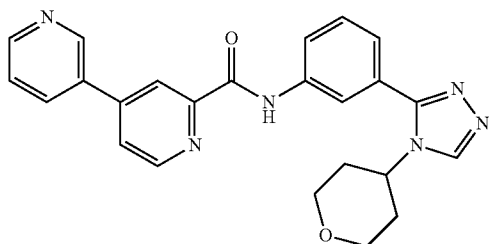
N-(3-(4-(tetrahydro-2H-pyran-4-yl)-4H-1,2,4-triazol-3-yl)phenyl)-3,4'-bipyridine-2'-carboxamide
