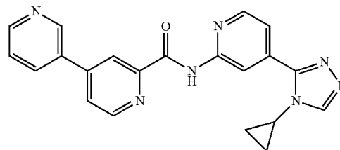
N-(4-(4-cyclopropyl-4H-1,2,4-triazol-3-yl)pyridin-2-yl)-3,4'-bipyridine-2'-carboxamide
