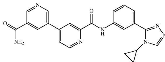
N2'-(3-(4-cyclopropyl-4H-1,2,4-triazol-3-yl)phenyl)-3,4'-bipyridine-2',5'-dicarboxamide
