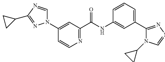
4-(3-cyclopropyl-1H-1,2,4-triazol-1-yl)-N-(3-(4-cyclopropyl-4H-1,2,4-triazol-3-yl)phenyl)picolinamide
