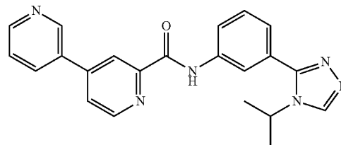
N-(3-(4-isopropyl-4H-1,2,4-triazol-3-yl)phenyl)-3,4'-bipyridine-2'-carboxamide
