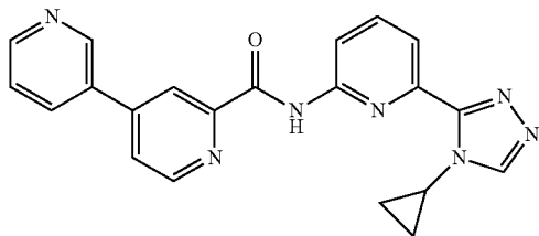
N-(6-(4-cyclopropyl-4H-1,2,4-triazol-3-yl)pyridin-2-yl)-3,4'-bipyridine-2'-carboxamide
