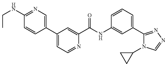
N-(3-(4-cyclopropyl-4H-1,2,4-triazol-3-yl)phenyl)-6-(ethylamino)-3,4'-bipyridine-2'-carboxamide
