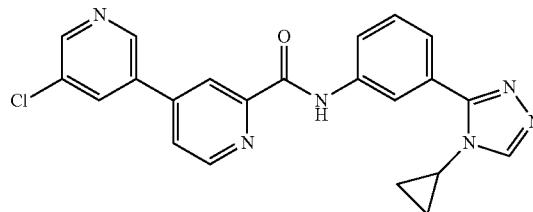
5-chloro-N-(3-(4-cyclopropyl-4H-1,2,4-triazol-3-yl)phenyl)-3,4'-bipyridine-2'-carboxamide
