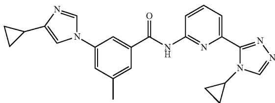
3-(4-cyclopropyl-1H-imidazol-1-yl)-N-(6-(4-cyclopropyl-4H-1,2,4-triazol-3-yl)pyridin-2-yl)-5-methylbenzamide
