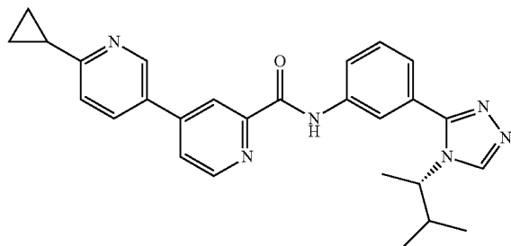
(S)-6-cyclopropyl-N-(3-(4-(3-methylbutan-2-yl)-4H-1,2,4-triazol-3-yl)phenyl)-3,4'-bipyridine-2'-carboxamide
