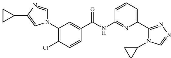
4-chloro-3-(4-cyclopropyl-1H-imidazol-1-yl)-N-(6-(4-cyclopropyl-4H-1,2,4-triazol-3-yl)pyridin-2-yl)benzamide
