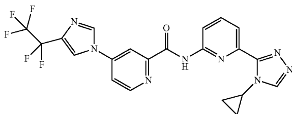
N-(6-(4-cyclopropyl-4H-1,2,4-triazol-3-yl)pyridin-2-yl)-4-(4-(perfluoroethyl)-1H-imidazol-1-yl)picolinamide
