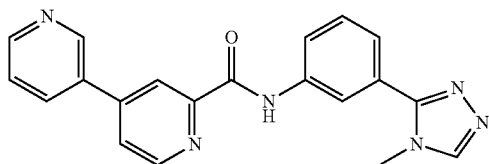
N-(3-(4-methyl-4H-1,2,4-triazol-3-yl)phenyl)-3,4'-bipyridine-2'-carboxamide
