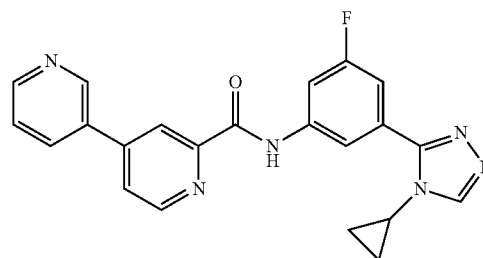
N-(3-(4-cyclopropyl-4H-1,2,4-triazol-3-yl)-5-fluorophenyl)-3,4'-bipyridine-2'-carboxamide
