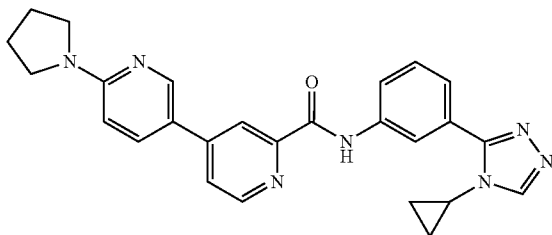
N-(3-(4-cyclopropyl-4H-1,2,4-triazol-3-yl)phenyl)-6-(pyrrolidin-1-yl)-3,4'-bipyridine-2'-carboxamide
