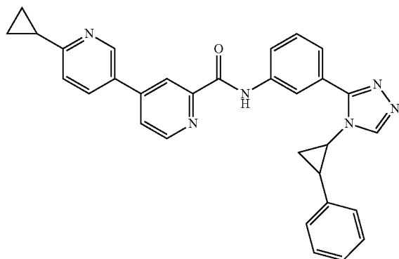
6-cyclopropyl-N-(3-(4-(2-phenylcyclopropyl)-4H-1,2,4-triazol-3-yl)phenyl)-3,4'-bipyridine-2'-carboxamide
