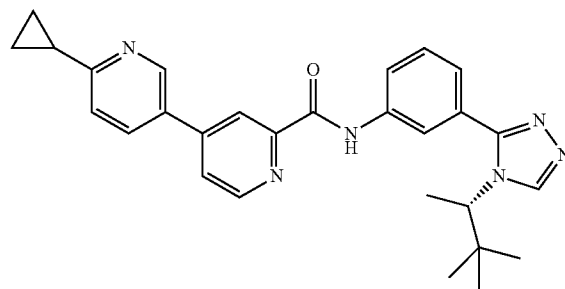
(S)-6-cyclopropyl-N-(3-(4-(3,3-dimethylbutan-2-yl)-4H-1,2,4-triazol-3-yl)phenyl)-3,4'-bipyridine-2'-carboxamide
