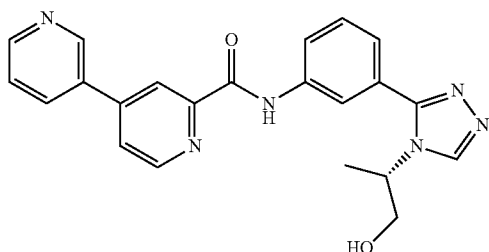
(S)-N-(3-(4-(1-hydroxypropan-2-yl)-4H-1,2,4-triazol-3-yl)phenyl)-3,4'-bipyridine-2'-carboxamide
