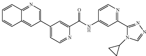
N-(2-(4-cyclopropyl-4H-1,2,4-triazol-3-yl)pyridin-4-yl)-4-(quinolin-3-yl)picolinamide
