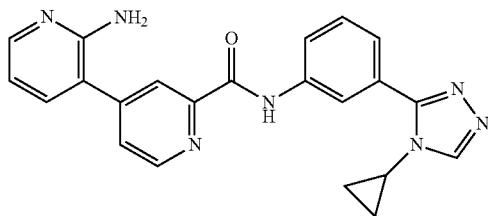
2-amino-N-(3-(4-cyclopropyl-4H-1,2,4-triazol-3-yl)phenyl)-3,4'-bipyridine-2'-carboxamide
