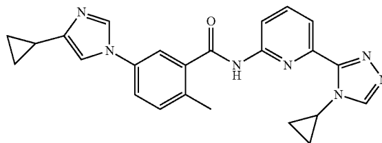
5-(4-cyclopropyl-1H-imidazol-1-yl)-N-(6-(4-cyclopropyl-4H-1,2,4-triazol-3-yl)pyridin-2-yl)-2-methylbenzamide
