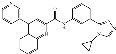
N-(3-(4-cyclopropyl-4H-1,2,4-triazol-3-yl)phenyl)-4-(pyridin-3-yl)quinoline-2-carboxamide
