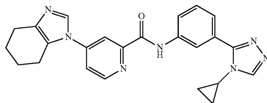
N-(3-(4-cyclopropyl-4H-1,2,4-triazol-3-yl)phenyl)-4-(4,5,6,7-tetrahydro-1H-benzo[d]imidazol-1-yl)picolinamide
