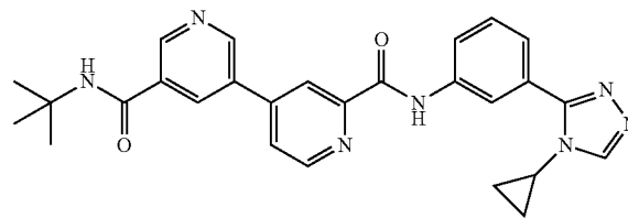
N5-tert-butyl-N2'-(3-(4-cyclopropyl-4H-1,2,4-triazol-3-yl)phenyl)-3,4'-bipyridine-2',5-dicarboxamide
