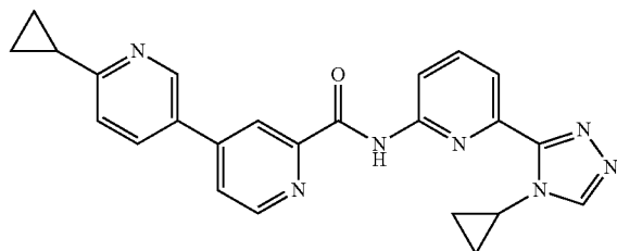
6-cyclopropyl-N-(6-(4-cyclopropyl-4H-1,2,4-triazol- 3-yl)pyridin-2-yl)-3,4'-bipyridine-2'-carboxamide
