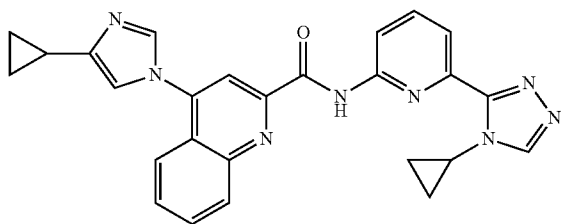
4-(4-cyclopropyl-1H-imidazol-1-yl)-N-(6-(4-cyclopropyl-4H-1,2,4-triazol-3-yl)pyridin-2-yl)quinoline-2-carboxamide
