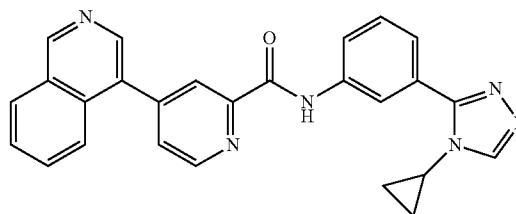
N-(3-(4-cyclopropyl-4H-1,2,4-triazol-3-yl)phenyl)-4-(isoquinolin-4-yl)picolinamide
