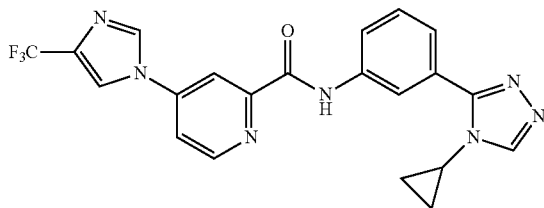
N-(3-(4-cyclopropyl-4H-1,2,4-triazol-3-yl)phenyl)-4-(4-(trifluoromethyl)-1H-imidazol-1-yl)picolinamide
