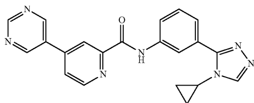
N-(3-(4-cyclopropyl-4H-1,2,4-triazol-3-yl)phenyl)- 4-(pyrimidin-5-yl)picolinamide
