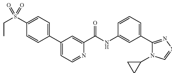
N-(3-(4-cyclopropyl-4H-1,2,4-triazol-3-yl)phenyl)- 4-(4-(ethylsulfonyl)-phenyl)picolinamide
