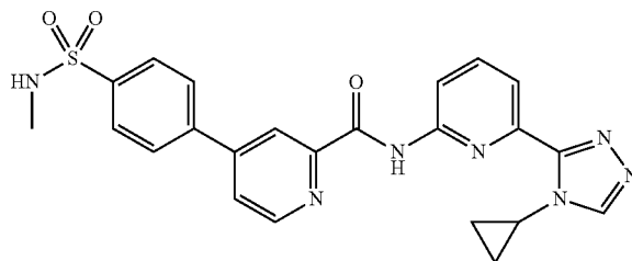
N-(6-(4-cyclopropyl-4H-1,2,4-triazol-3-yl)pyridin-2-yl)-4-(4-(N-methylsulfamoyl)phenyl)picolinamide
