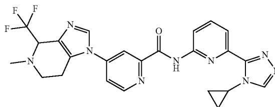
N-(6-(4-cyclopropyl-4H-1,2,4-triazol-3-yl)pyridin-2-yl)-4-(5-methyl-4-(trifluoromethyl)-4,5,6,7-tetrahydro-1H-imidazo[4,5-c]pyridin-1-yl)picolinamide
