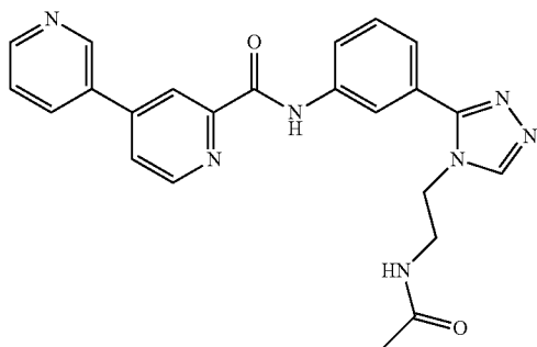
N-(3-(4-(2-acetamidoethyl)-4H-1,2,4-triazol-3-yl)phenyl)-3,4'-bipyridine-2'-carboxamide
