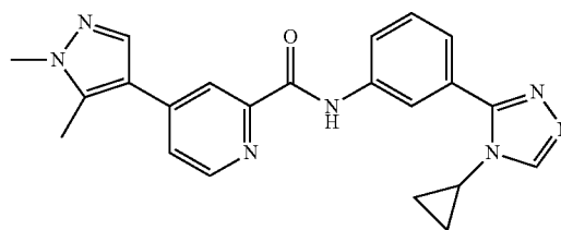
N-(3-(4-cyclopropyl-4H-1,2,4-triazol-3-yl)phenyl)-4-(1,5-dimethyl-1H-pyrazol-4-yl)picolinamide
