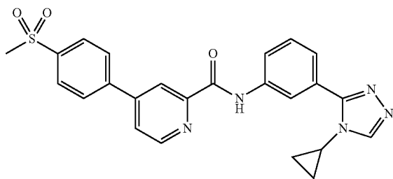
N-(3-(4-cyclopropyl-4H-1,2,4-triazol-3-yl)phenyl)-4-(4-(methylsulfonyl)phenyl)picolinamide
