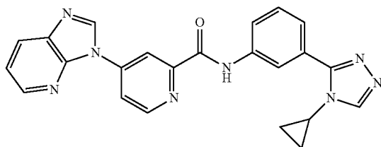
N-(3-(4-cyclopropyl-4H-1,2,4-triazol-3-yl)phenyl)-4-(3H-imidazo[4,5-b]pyridin-3-yl)picolinamide
