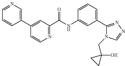
N-(3-(4-((1-hydroxycyclopropyl)methyl)-4H-1,2,4-triazol-3-yl)phenyl)-3,4'-bipyridine-2'-carboxamide
