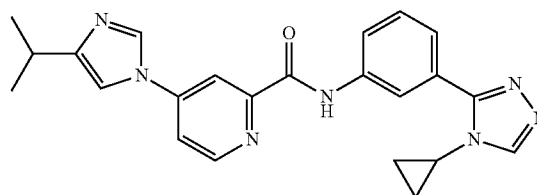
N-(3-(4-cyclopropyl-4H-1,2,4-triazol-3-yl)phenyl)-4-(4-isopropyl-1H-imidazol-1-yl)picolinamide
