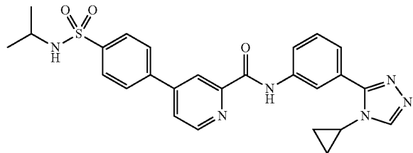
N-(3-(4-cyclopropyl-4H-1,2,4-triazol-3-yl)phenyl)- 4-(4-(N-isopropylsulfonyl)-phenyl)picolinamide
