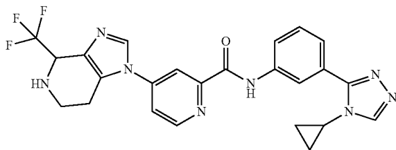
N-(3-(4-cyclopropyl-4H-1,2,4-triazol-3-yl)phenyl)-4-(4-(trifluoromethyl)-4,5,6,7-tetrahydro-1H-imidazo[4,5-c]pyridin-1-yl)picolinamide
