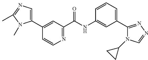
N-(3-(4-cyclopropyl-4H-1,2,4-triazol-3-yl)phenyl)-4-(1,2-dimethyl-1H-imidazol-5-yl)picolinamide
