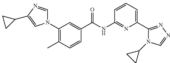
3-(4-cyclopropyl-1H-imidazol-1-yl)-N-(6-(4-cyclopropyl-4H-1,2,4-triazol-3-yl)pyridin-2-yl)-4-methylbenzamide
