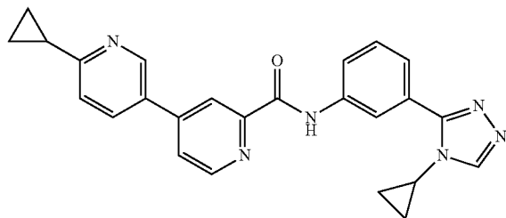
6-cyclopropyl-N-(3-(4-cyclopropyl-4H-1,2,4-triazol- 3-yl)phenyl)-3,4'-bipyridine-2'-carboxamide
