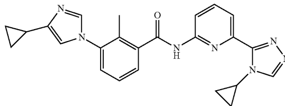
3-(4-cyclopropyl-1H-imidazol-1-yl)-N-(6-(4-cyclopropyl-4H-1,2,4-triazol-3-yl)pyridin-2-yl)-2-methylbenzamide
