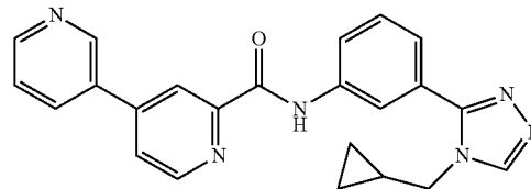
N-(3-(4-(cyclopropylmethyl)-4H-1,2,4-triazol-3-yl)phenyl)-3,4'-bipyridine-2'-carboxamide
