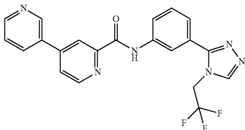
N-(3-(4-(2,2,2-trifluoroethyl)-4H-1,2,4-triazol-3-yl)phenyl)-3,4'-bipyridine-2'-carboxamide
