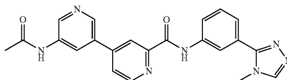
5-acetamido-N-(3-(4-methyl-4H-1,2,4-triazol-3-yl)phenyl)-3,4'-bipyridine-2'-carboxamide
