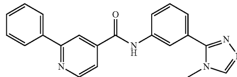
N-(3-(4-ethyl-4H-1,2,4-triazol-3-yl)phenyl)-2-phenylisonicotinamide
