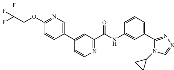
N-(3-(4-cyclopropyl-4H-1,2,4-triazol-3-yl)phenyl)-6-(2,2,2-trifluoroethoxy)-3,4'-bipyridine-2'-carboxamide
