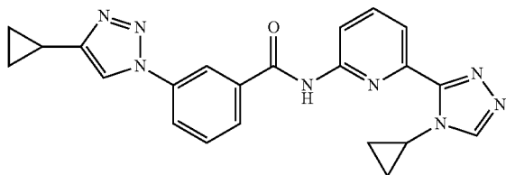
3-(4-cyclopropyl-1H-1,2,3-triazol-1-yl)-N-(6-(4-cyclopropyl-4H-1,2,4-triazol-3-yl)pyridin-2-yl)benzamide
