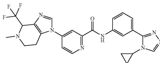
N-(3-(4-cyclopropyl-4H-1,2,4-triazol-3-yl)phenyl)-4-(5-methyl-4-(trifluoromethyl)-4,5,6,7-tetrahydro-1H-imidazo[4,5-c]pyridin-1-yl)picolinamide
