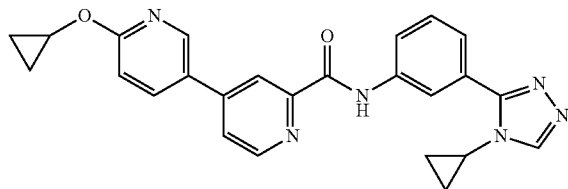
6-cyclopropoxy-N-(3-(4-cyclopropyl-4H-1,2,4-triazol-3-yl)phenyl)-3,4'-bipyridine-2'-carboxamide
