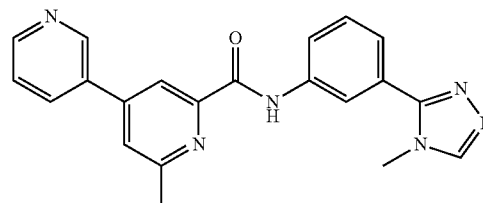
6'-methyl-N-(3-(4-methyl-4H-1,2,4-triazol-3-yl)phe- nyl)-3,4'-bipyridine-2'-carboxamide
