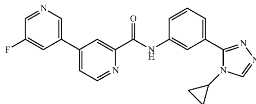
N-(3-(4-cyclopropyl-4H-1,2,4-triazol-3-yl)phenyl)-5-fluoro-3,4'-bipyridine-2'-carboxamide
