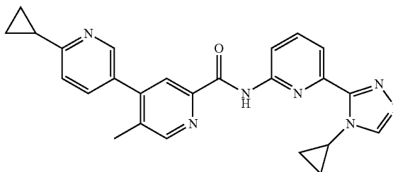
6-cyclopropyl-N-(6-(4-cyclopropyl-4H-1,2,4-triazol-3-yl)pyridin-2-yl)-5'-methyl-3,4'-bipyridine-2'-carboxamide
