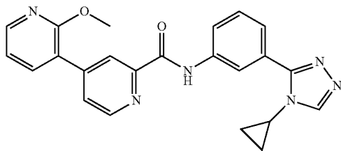
N-(3-(4-cyclopropyl-4H-1,2,4-triazol-3-yl)phenyl)-2-methoxy-3,4'-bipyridine-2'-carboxamide
