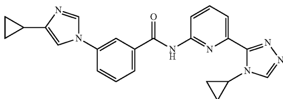
3-(4-cyclopropyl-1H-imidazol-1-yl)-N-(6-(4-cyclopropyl-4H-1,2,4-triazol-3-yl)pyridin-2-yl)benzamide
