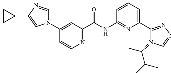
(S)-4-(4-cyclopropyl-1H-imidazol-1-yl)-N-(3-(4-(3-methylbutan-2-yl)-4H-1,2,4-triazol-3-yl)phenyl)picolinamide
