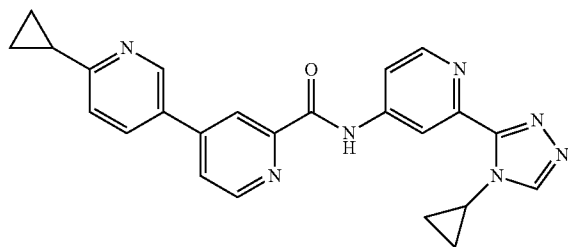
6-cyclopropyl-N-(2-(4-cyclopropyl-4H-1,2,4-triazol-3-yl)pyridin-4-yl)-3,4'-bipyridine-2'-carboxamide
