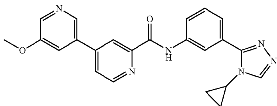
N-(3-(4-cyclopropyl-4H-1,2,4-triazol-3-yl)phenyl)-5-methoxy-3,4'-bipyridine-2'-carboxamide
