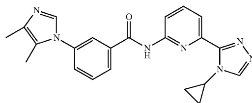
N-(6-(4-cyclopropyl-4H-1,2,4-triazol-3-yl)pyridin-2-yl)-3-(4,5-dimethyl-1H-imidazol-1-yl)benzamide
