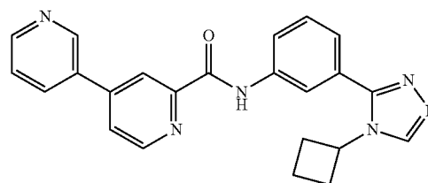
N-(3-(4-(cyclobutyl)-4H-1,2,4-triazol-3-yl)phenyl)-3,4'-bipyridine-2'-carboxamide
