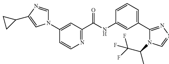
(S)-4-(4-cyclopropyl-1H-imidazol-1-yl)-N-(3-(4-(1,1,1-trifluoropropan-2-yl)-4H-1,2,4-triazol-3-yl)phenyl)picolinamide
