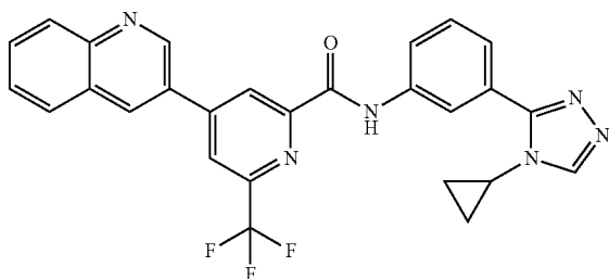
N-(3-(4-cyclopropyl-4H-1,2,4-triazol-3-yl)phenyl)-4-(quinolin-3-yl)-6-(trifluoromethyl)picolinamide
