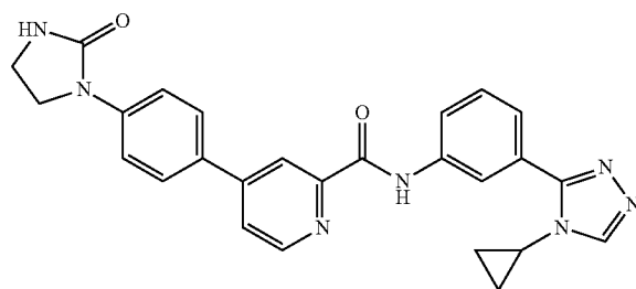
N-(3-(4-cyclopropyl-4H-1,2,4-triazol-3-yl)phenyl)-4-(4-(2-oxoimidazolidin-1-yl)phenyl)picolinamide
