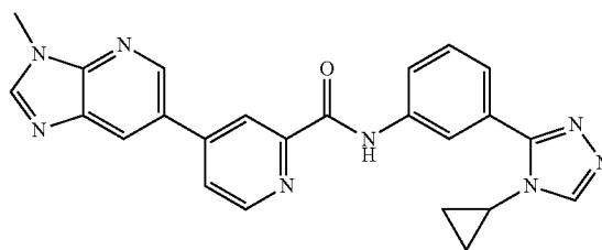
N-(3-(4-cyclopropyl-4H-1,2,4-triazol-3-yl)phenyl)-4-(3-methyl-3H-imidazo[4,5-b]pyridin-6-yl)picolinamide
