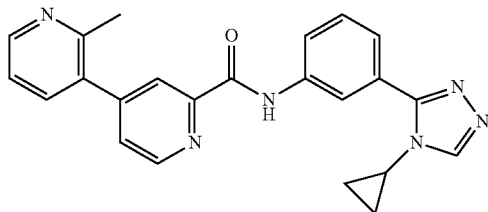
N-(3-(4-cyclopropyl-4H-1,2,4-triazol-3-yl)phenyl)-2-methyl-3,4'-bipyridine-2'-carboxamide
