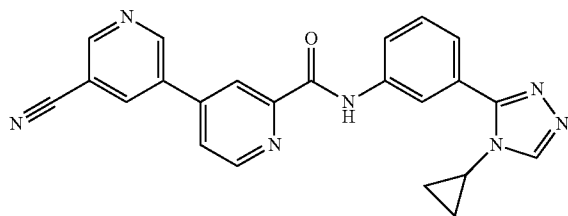
5-cyano-N-(3-(4-cyclopropyl-4H-1,2,4-triazol-3-yl)phenyl)-3,4'-bipyridine-2'-carboxamide
