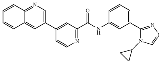
N-(3-(4-cyclopropyl-4H-1,2,4-triazol-3-yl)phenyl)-4-(quinolin-3-yl)picolinamide
