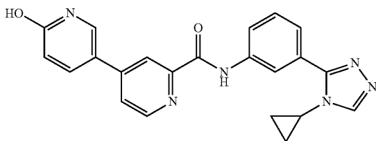
N-(3-(4-cyclopropyl-4H-1,2,4-triazol-3-yl)phenyl)- 6-hydroxy-3,4'-bipyridine-2'-carboxamide
