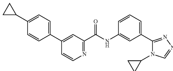
N-(3-(4-cyclopropyl-4H-1,2,4-triazol-3-yl)phenyl)-4-(4-cyclopropylphenyl)picolinamide
