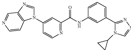
N-(3-(4-cyclopropyl-4H-1,2,4-triazol-3-yl)phenyl)-4-(1H-imidazo[4,5-c]pyridin-1-yl)picolinamide
