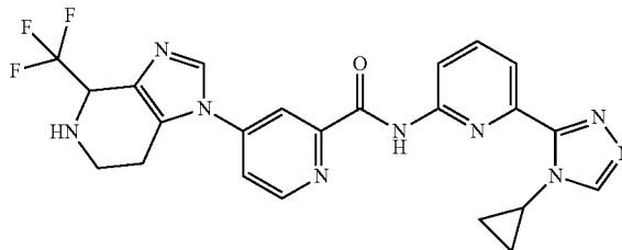
N-(6-(4-cyclopropyl-4H-1,2,4-triazol-3-yl)pyridin-2-yl)-4-(4-(trifluoromethyl)-4,5,6,7-tetrahydro-1H-imidazo[4,5-c]pyridin-1-yl)picolinamide
