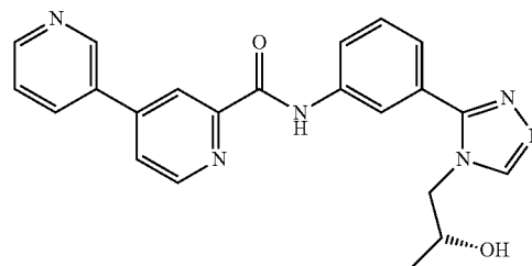
[0729] (R)-N-(3-(4-(2-hydroxypropyl)-4H-1,2,4-triazol-3-yl)phenyl)-3,4'-bipyridine-2'-carboxamide
