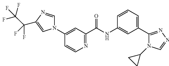
N-(3-(4-cyclopropyl-4H-1,2,4-triazol-3-yl)phenyl)- 4-(4-(perfluoroethyl)-1H-imidazol-1-yl)picolinamide
