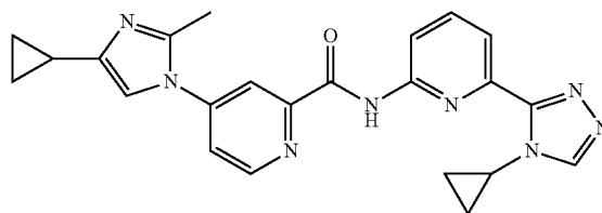
4-(4-cyclopropyl-2-methyl-1H-imidazol-1-yl)-N-(6-(4-cyclopropyl-4H-1,2,4-triazol-3-yl)pyridin-2-yl)picolinamide
