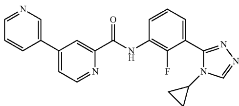
N-(3-(4-cyclopropyl-4H-1,2,4-triazol-3-yl)-2-fluorophenyl)-3,4'-bipyridine-2'-carboxamide
