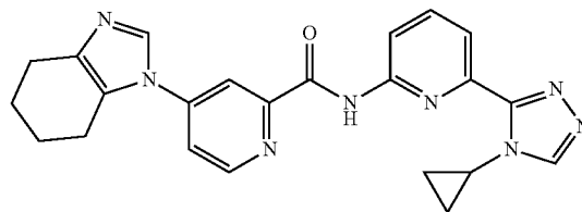
N-(6-(4-cyclopropyl-4H-1,2,4-triazol-3-yl)pyridin-2-yl)-4-(4,5,6,7-tetrahydro-1H-benzo[d]imidazol-1-yl)picolinamide
