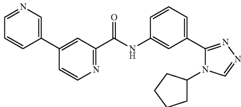
N-(3-(4-cyclopentyl-4H-1,2,4-triazol-3-yl)phenyl)-3,4'-bipyridine-2'-carboxamide
