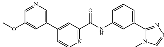
5-methoxy-N-(3-(4-methyl-4H-1,2,4-triazol-3-yl)phenyl)-3,4'-bipyridine-2'-carboxamide
