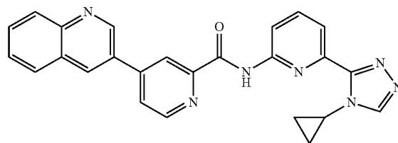
N-(6-(4-cyclopropyl-4H-1,2,4-triazol-3-yl)pyridin-2-yl)-4-(quinolin-3-yl)picolinamide
