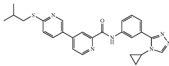
N-(3-(4-cyclopropyl-4H-1,2,4-triazol-3-yl)phenyl)-6-(isobutylthio)-3,4'-bipyridine-2'-carboxamide
