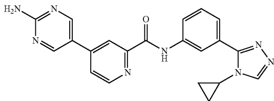
4-(2-aminopyrimidin-5-yl)-N-(3-(4-cyclopropyl-4H- 1,2,4-triazol-3-yl)phenyl)picolinamide
