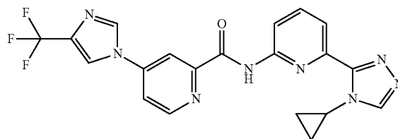
N-(6-(4-cyclopropyl-4H-1,2,4-triazol-3-yl)pyridin-2-yl)-4-(4-(trifluoromethyl)-1H-imidazol-1-yl)picolinamide
