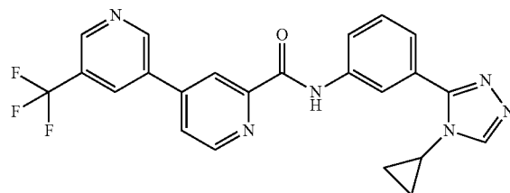
N-(3-(4-cyclopropyl-4H-1,2,4-triazol-3-yl)phenyl)-5-(trifluoromethyl)-3,4'-bipyridine-2'-carboxamide
