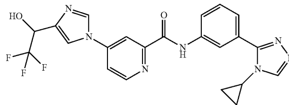
N-(3-(4-cyclopropyl-4H-1,2,4-triazol-3-yl)phenyl)-4-(4-(2,2,2-trifluoro-1-hydroxyethyl)-1H-imidazol-1-yl)picolinamide
