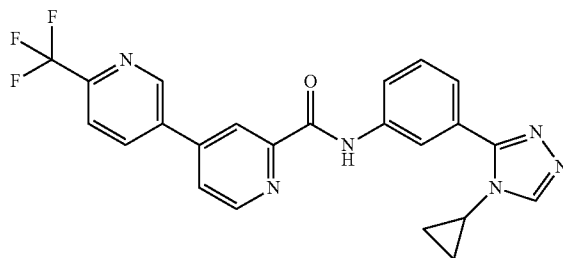
N-(3-(4-cyclopropyl-4H-1,2,4-triazol-3-yl)phenyl)- 6-(trifluoromethyl)-3,4'-bipyridine-2'-carboxamide
