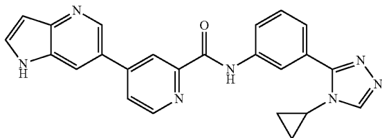
N-(3-(4-cyclopropyl-4H-1,2,4-triazol-3-yl)phenyl)-4-(1H-pyrrolo[3,2-b]pyridin-6-yl)picolinamide
