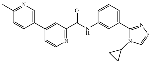
N-(3-(4-cyclopropyl-4H-1,2,4-triazol-3-yl)phenyl)- 6-methyl-3,4'-bipyridine-2'-carboxamide
