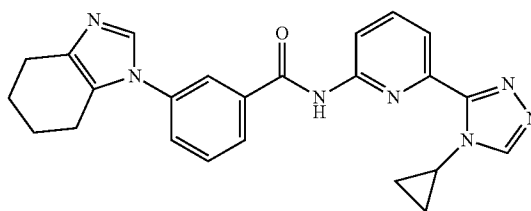
N-(6-(4-cyclopropyl-4H-1,2,4-triazol-3-yl)pyridin-2-yl)-3-(4,5,6,7-tetrahydro-1H-benzo[d]imidazol-1-yl)benzamide
