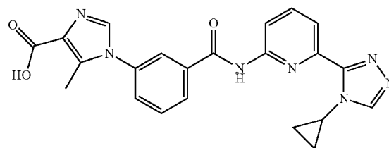
1-(3-(6-(4-cyclopropyl-4H-1,2,4-triazol-3-yl)pyridin-2-ylcarbamoyl)phenyl)-5-methyl-1H-imidazole-4-carboxylic acid
