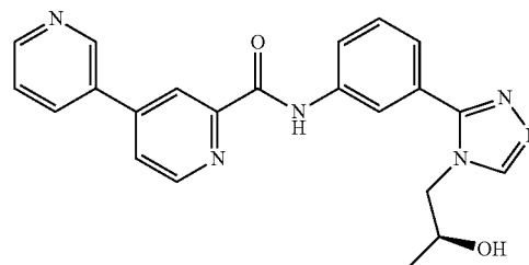
(S)-N-(3-(4-(2-hydroxypropyl)-4H-1,2,4-triazol-3-yl)phenyl)-3,4'-bipyridine-2'-carboxamide
