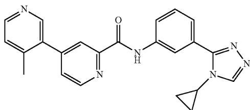
N-(3-(4-cyclopropyl-4H-1,2,4-triazol-3-yl)phenyl)-4-methyl-3,4'-bipyridine-2'-carboxamide
