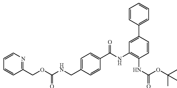
1,1-dimethylethyl 3-(((4-(((pyridin-2-ylmethyl)oxy)carbonyl)amino)methyl)phenyl)carbonyl)amino]biphenyl-4-yl]carbamate
