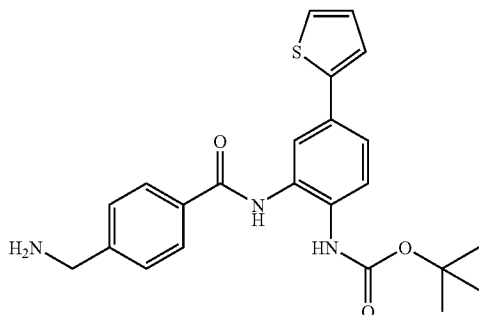
1,1-dimethylethyl[2-({[4-(aminomethyl)phenyl]carbonyl}amino)-4-(2-thienyl)phenyl]carbamate
