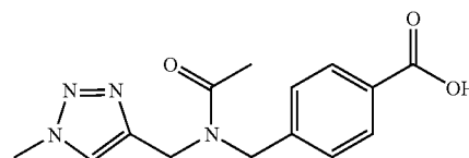
4-({Acetyl[1-methyl-1H-1,2,3-triazol-4-yl]methyl}amino)benzoic acid
