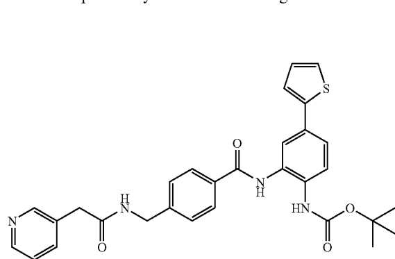
1,1-dimethylethyl[2-[[{(4-[[{(pyridin-3-ylacetyl)amino]methyl}phenyl)carbonyl]amino}-4-(2-thienyl)phenyl]carbamate
