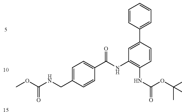
1,1-dimethylethyl[3-({[4-({(methoxy)carbonyl}amino)methyl]phenyl]carbonyl}amino)biphenyl-4-yl]carbamate
