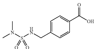
4-((dimethylamino)sulfonyl)aminomethylbenzoic acid
