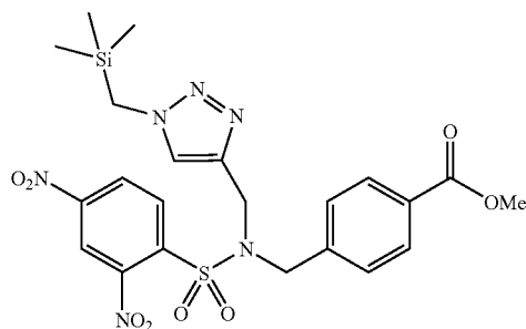
Methyl 4-({[1-((trimethylsilyl)methyl)-1H-1,2,3-triazol-4-yl]methyl}amino)benzoate
