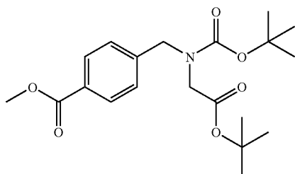
Methyl 4-tert-butoxycarbonyl(2-tert-butoxy-2-oxoethyl)amino]methyl]benzoate
