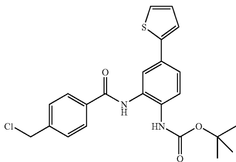
1,1-dimethylethyl[2-({[4-(chloromethyl)phenyl]carbonyl}amino)-4-(2-thienyl)phenyl]carbamate
