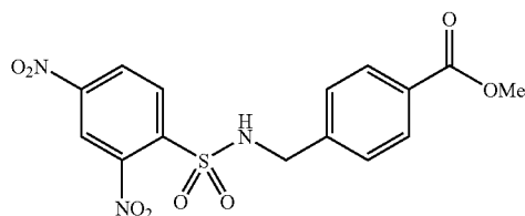
Methyl 4-({[(2,4-dinitrophenyl)sulfonyl]amino}methyl)benzoate
