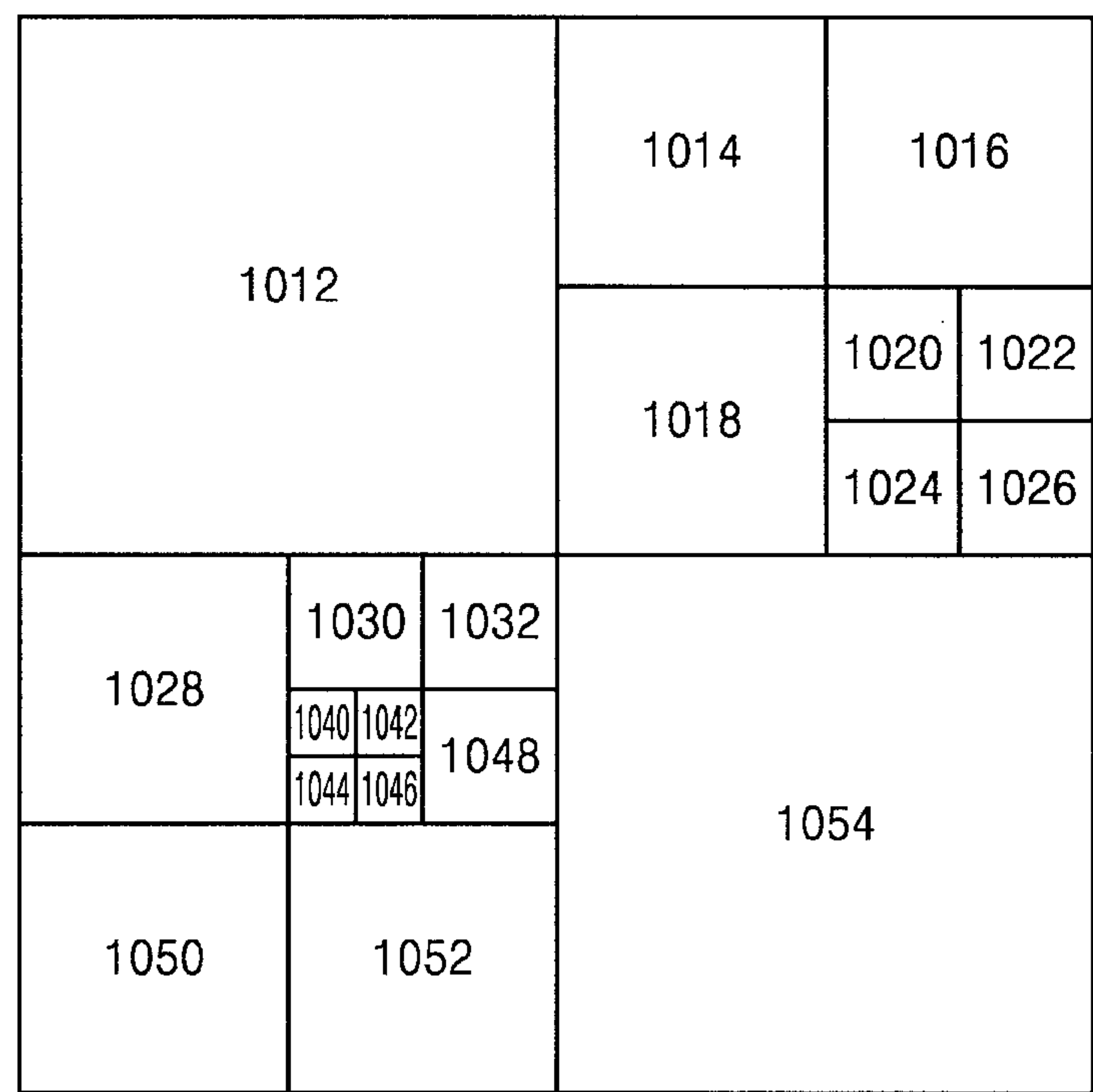
CODING UNIT (1010)
