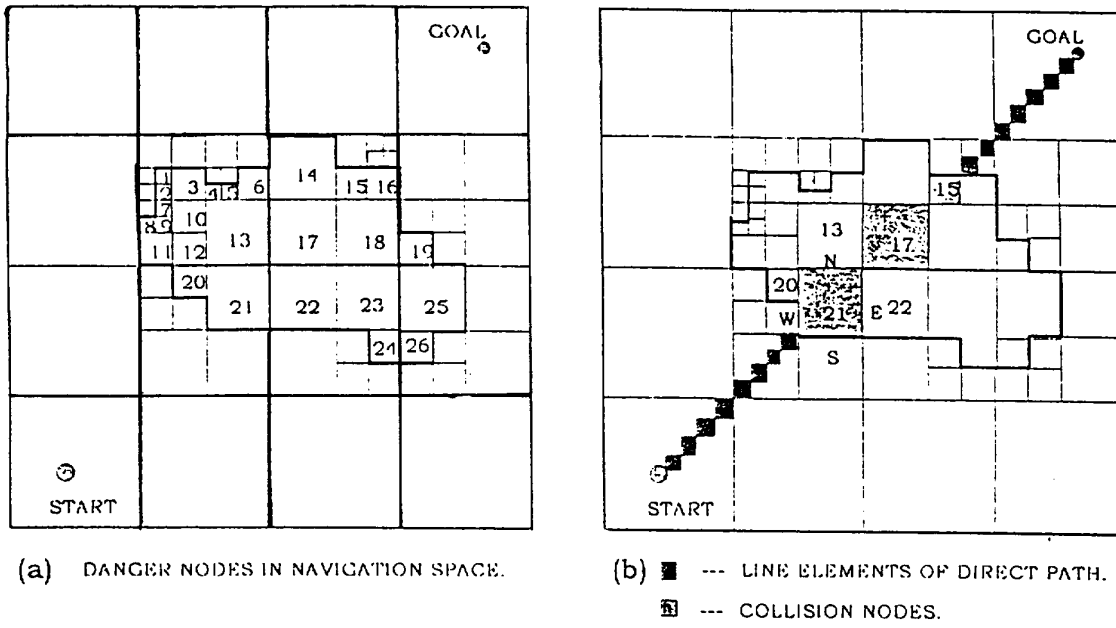
Figure 3. An example of navigation space with danger nodes.
