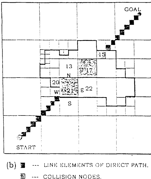
Figure 3. An example of navigation space with danger nodes.
