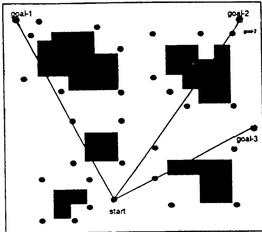
(a) A NAVIGATION SPACE WITH 32 WAYPOINTS.
