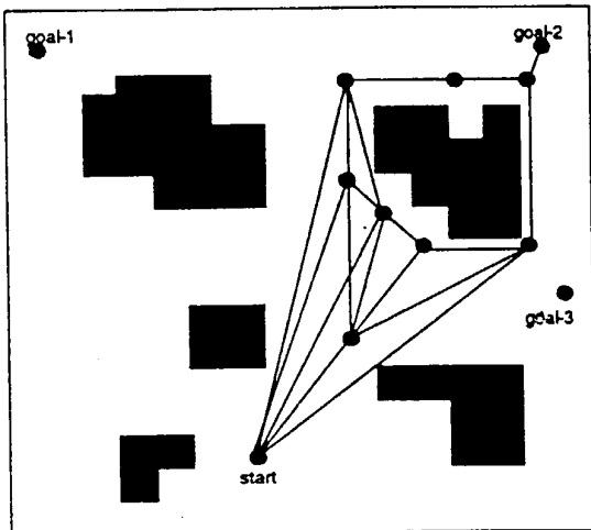
(c) PATH START TO GOAL-2, 10 WAYPOINTS.
