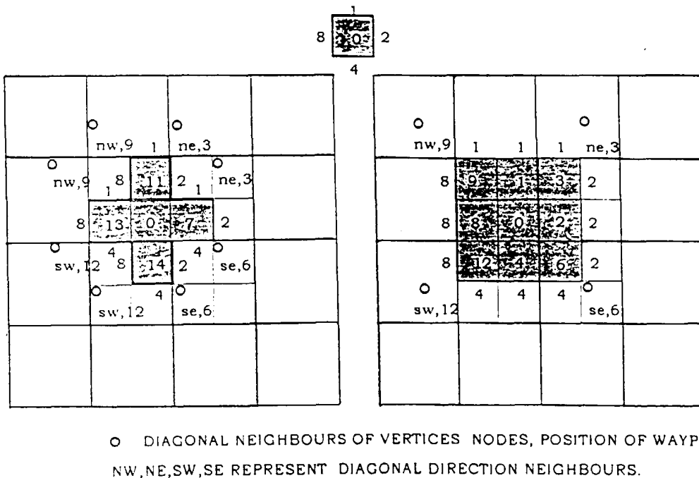
Figure 5. An example of using binary search of danger node list to determine the boundary nodes during dangerous zone expansion (dangerous zone refer to Figure 3).
