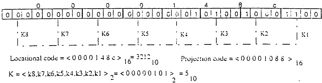
Figure 2. Bit interleave of locational code and 2-D, 3D projection.
