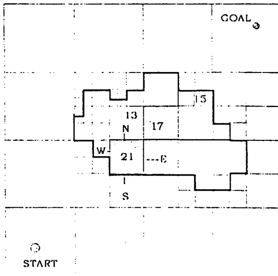
(a) EXPANSION FROM NODE 21 TO ITS FOUR MAIN DIRECTION NEIGHBOURS RECURSIVELY.
