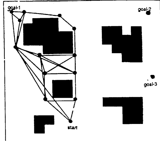
(b) PATH START TO GOAL-1, 13 WAYPOINTS.
