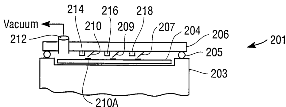
FIG. 2 (PRIOR ART)
