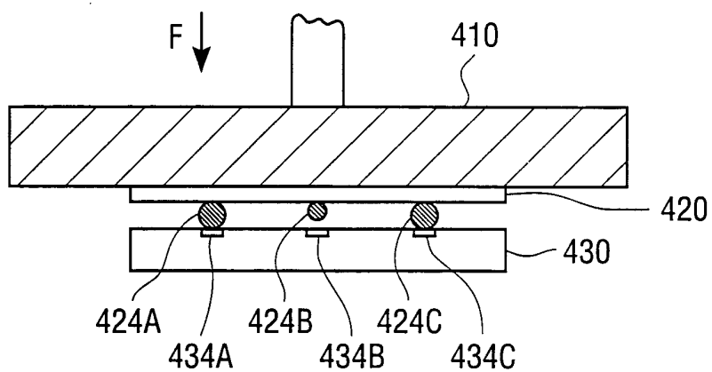
FIG. 4C (PRIOR ART)
