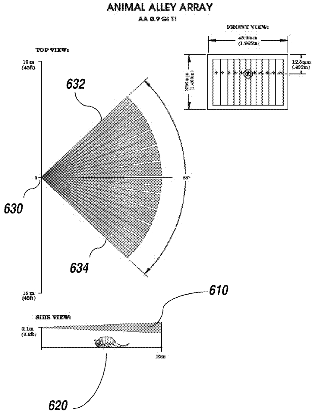
Fig. 6 (prior art)
