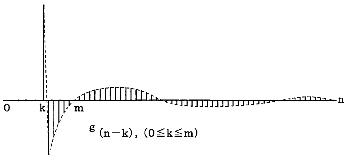
OPTIMUMLY APPROXIMATED IIR FILTER IMPULSE RESPONSE
