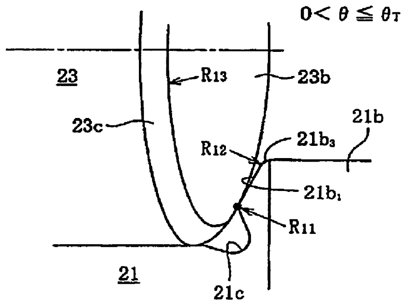
FIG. 11(PRIOR ART)
