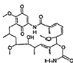
Geldanamycin
